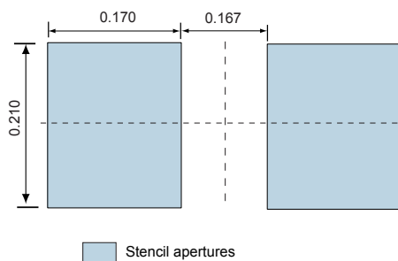
Figure 12. Stencil opening recommendations
