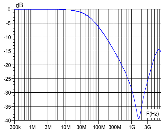
Figure 7. S21 attenuation
