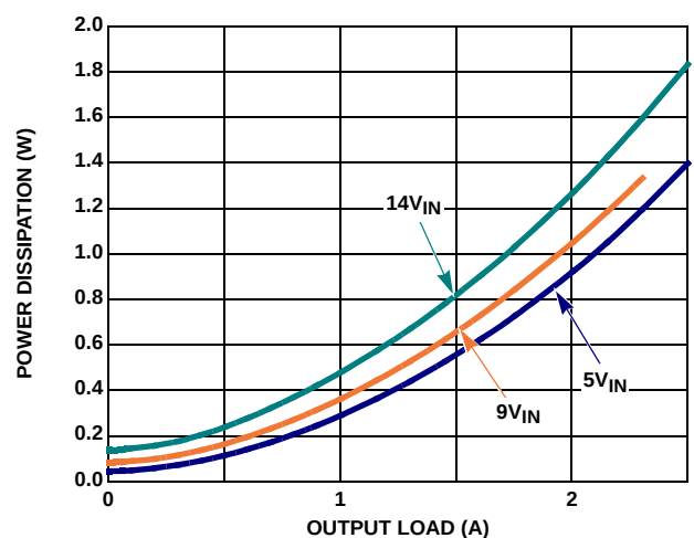
FIGURE 12. POWER DISSIPATION vs LOAD ( V_{OUT} = 0.6V , 500kHz)
