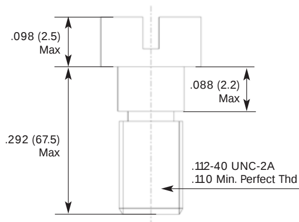
Part Number 8 MC JS 515 - Mil Spec M83513/05-15
