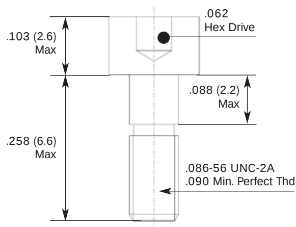
Part Number 8 MC JS 502 - Mil Spec M83513/05-02
