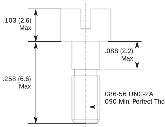
Part Number 8 MC JS 505 - Mil Spec M83513/05-05
