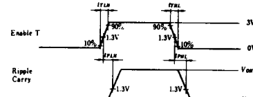
Waveform—3 t_{PLH} , t_{PHL} (Enable T→Ripple Carry)
