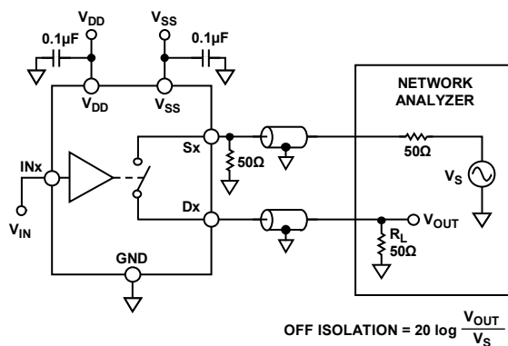
Figure 27. Off Isolation
