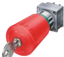
Mushroom diameter 40 mm, with CES key-operated switch
