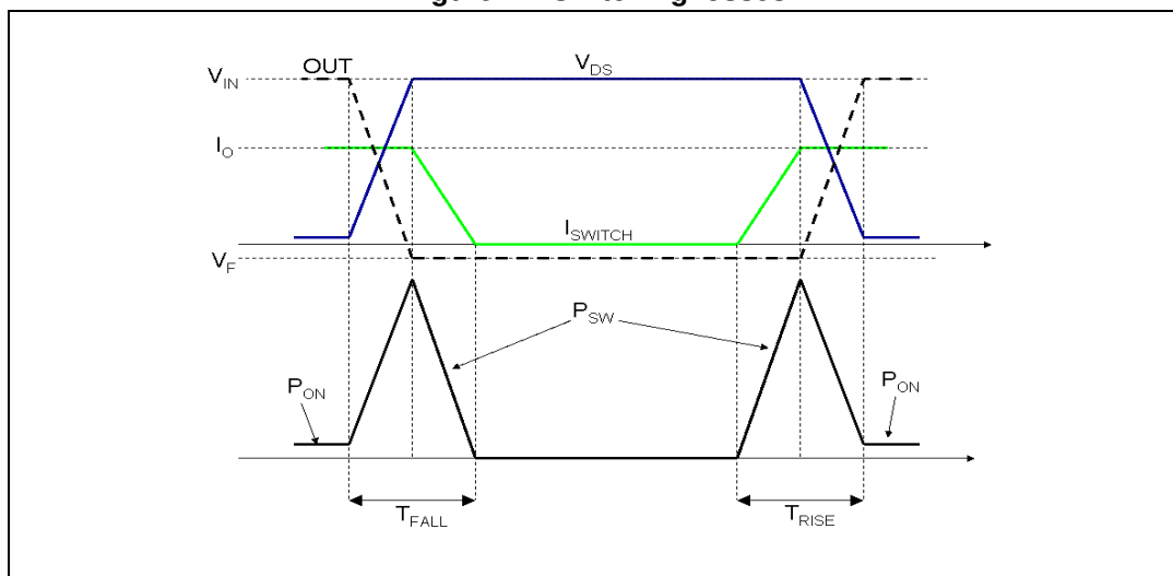
Figure 12. Switching losses
