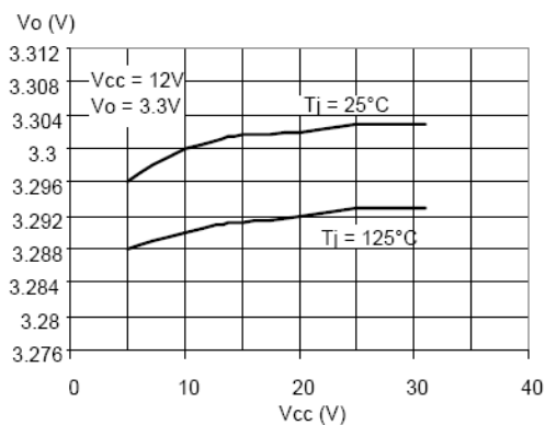
Figure 23. Line regulation
