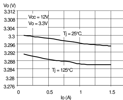
Figure 24. Load regulation
