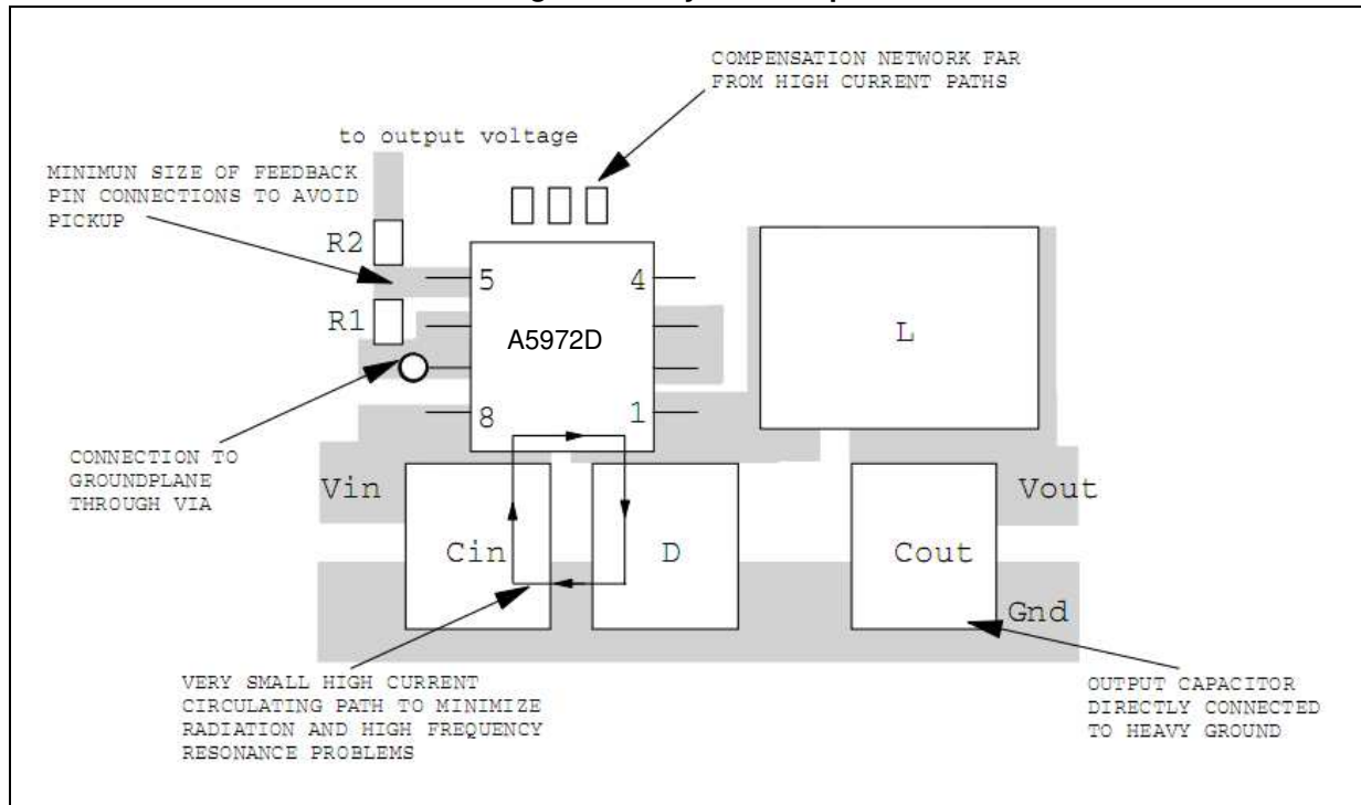
Figure 11. Layout example
