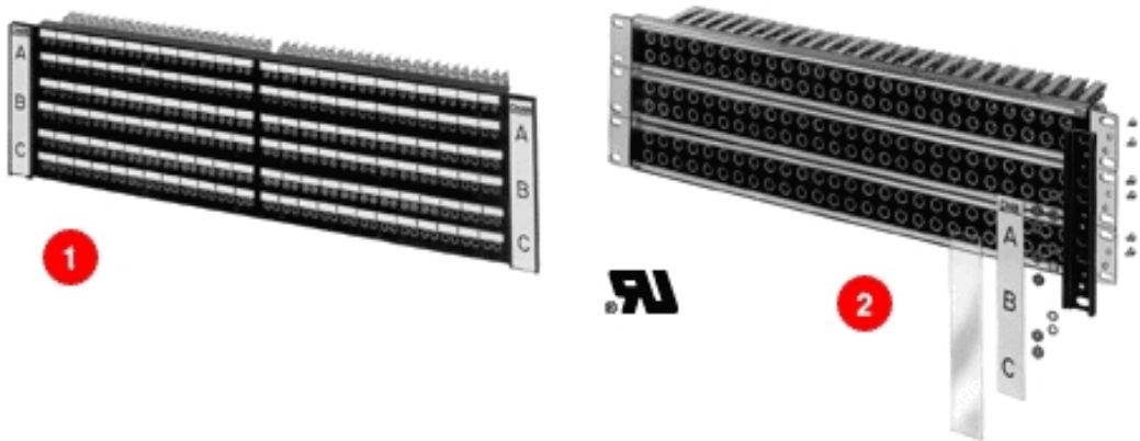
1. 3-row Jack Panels Assembly with DS323 X-Wide Designation Strip installed 2. Assembly sequence of DS323 X-Wide Designation Strip
