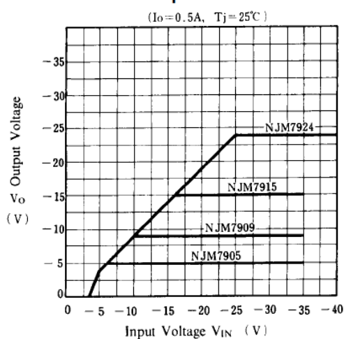
NJM7900 Output Characteristics
