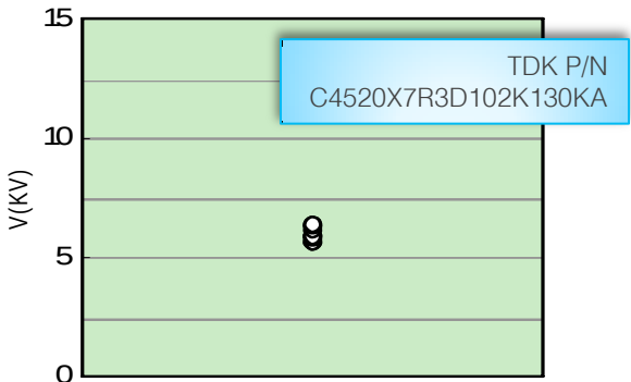
DC Breakdown Voltage
