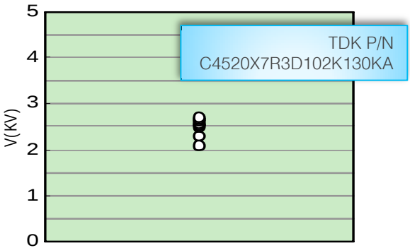
AC Breakdown Voltage
