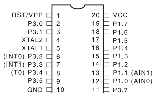
PDIP/SOIC
