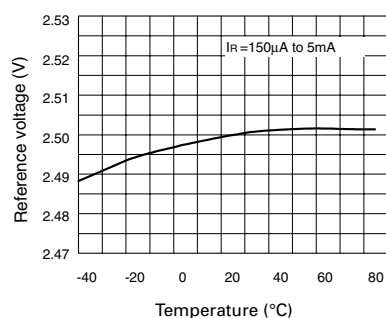
Temperature Drift
