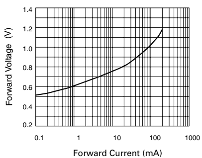
Forward Characteristics
