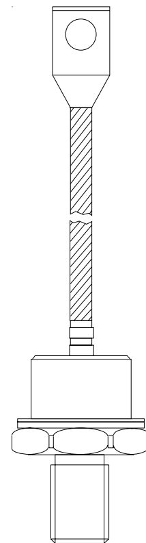
case style DO-205AC (DO-30)
