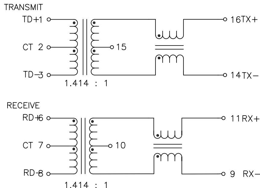
SCHEMATIC
