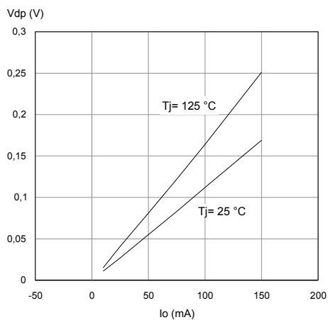
Figure 5. Drop Voltage vs. Output Current
