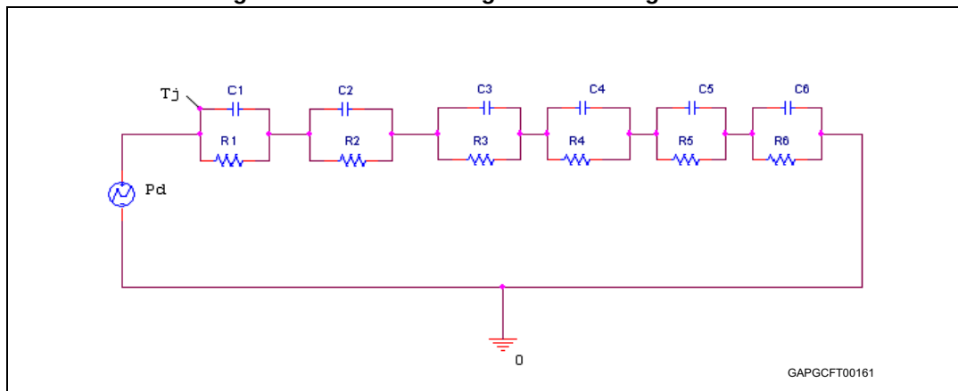
Figure 35. Thermal fitting model of Vreg in SO-20
