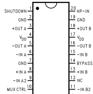
Figure 2. Top View See Package Number PW0020A for TSSOP See Package Number PWP0020A for Exposed-DAP HTSSOP
