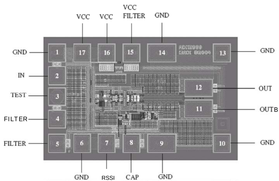
Figure 2.. Pad Layout
