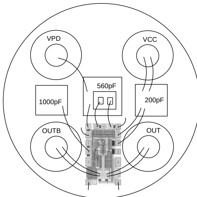
Figure 3. 5-Pin TO-46 w/External Photodiode Supply V_{PD}
