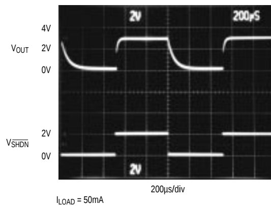
MAX8864 SHUTDOWN
