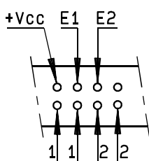
Solder pins
