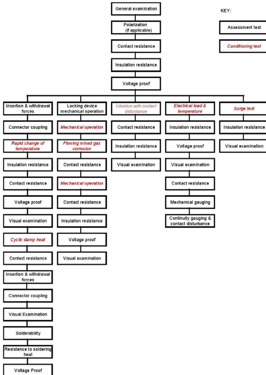
Figure 7 Reference Test Schedule Required for Modular Jacks, per IEC 60603-7 Series
