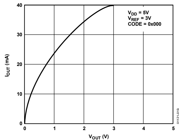
Figure 16. I_{OUT} at Zero Scale vs. V_{OUT}
