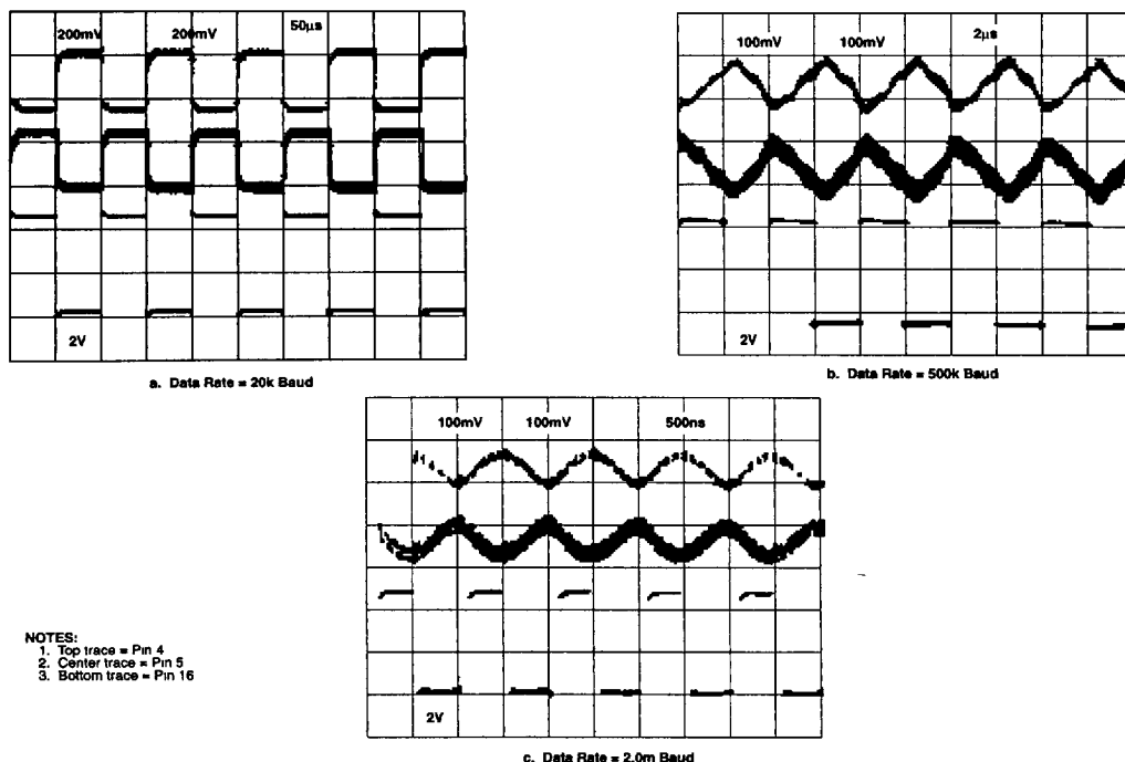
Figure 6. Phase Comparator (Pins 4 and 5) and FSK (Pin 16) Outputs
