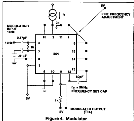
Figure 4. Modulator
