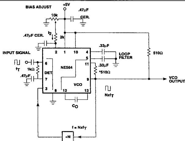
Figure 7. NE564 Phase-Locked Frequency Multiplier
