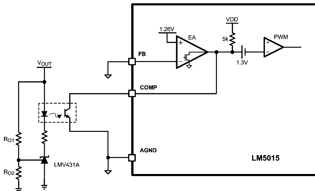
FIGURE 9. Conventional Isolated Feedback
