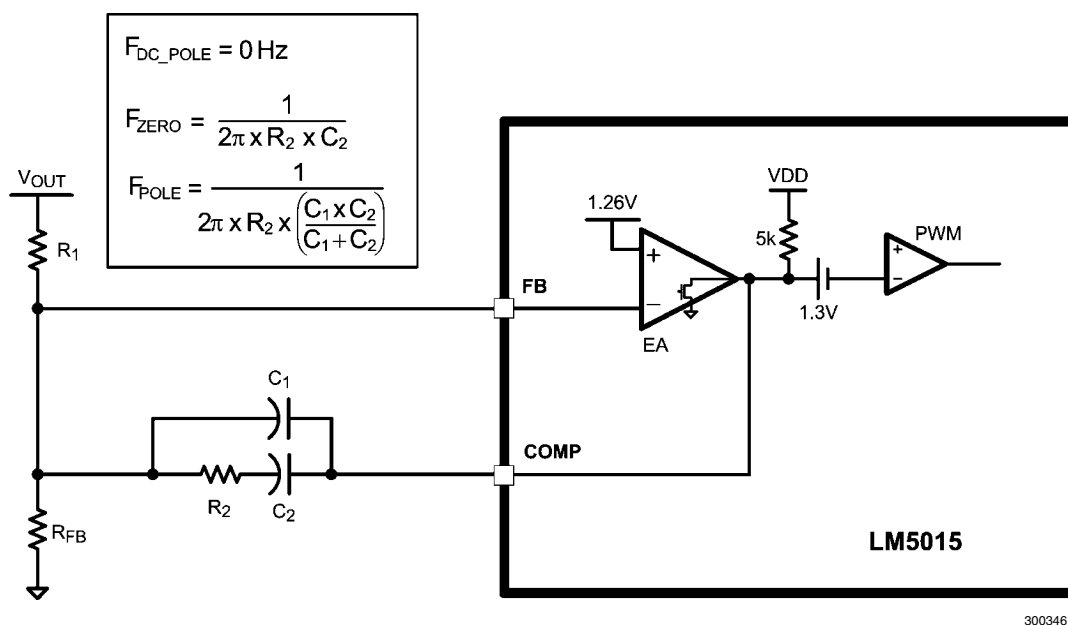
FIGURE 3. Type II Compensator
