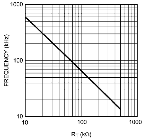
Fsw vs R RT
