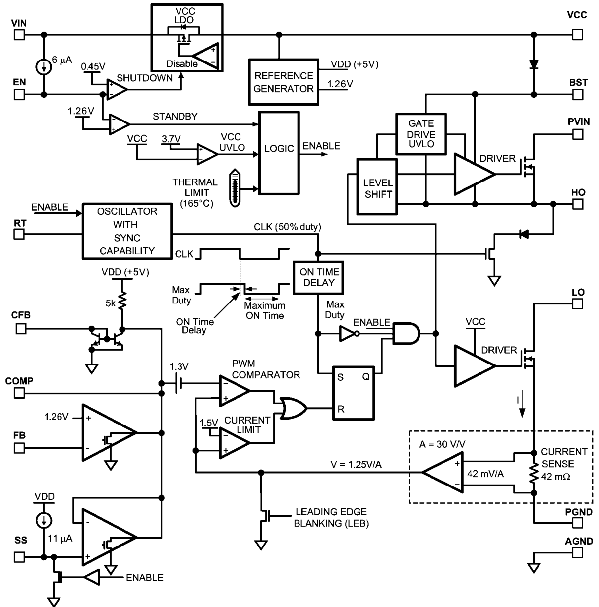
FIGURE 1. Block Diagram
