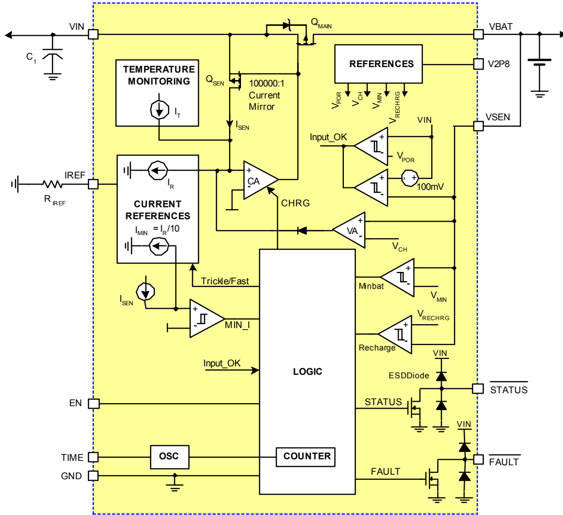
FIGURE 16. BLOCK DIAGRAM
