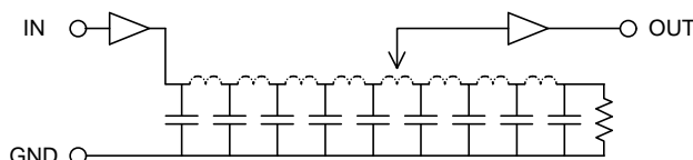
Functional Diagram
