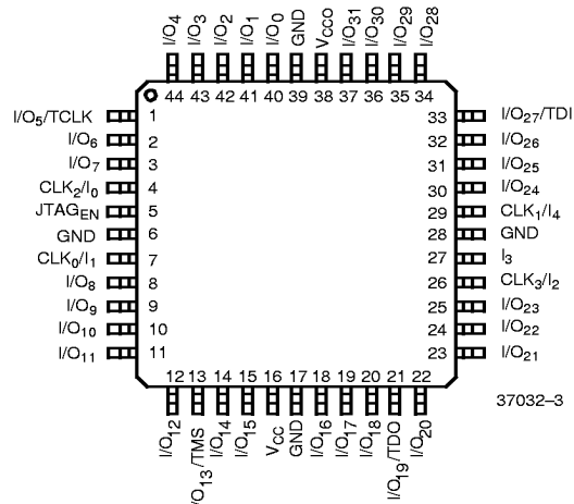
44-Pin TQFP Top View
