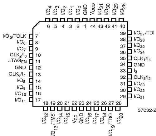
44-Pin PLCC Top View
