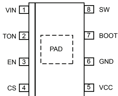
Pinout Diagram
