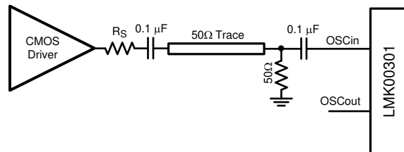
Figure 9-4. Driving OSCin With a Single-Ended Input
