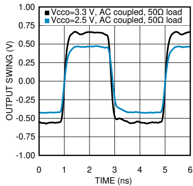
Figure 6-9. LVC MOS Output Swing at 250MHz
