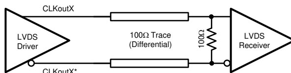
Figure 9-6. Differential LVDS Operation, DC Coupling, No Biasing by the Receiver
