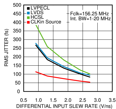
Figure 6-14. RMS Jitter vs CLKIn Slew Rate at 156.25MHz
