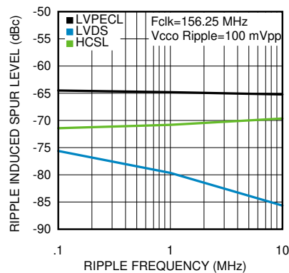
Figure 6-16. PSRR vs Ripple Frequency at 156.25MHz
