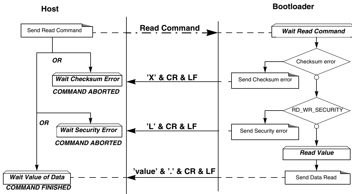
Figure 24-16. Read Flow
