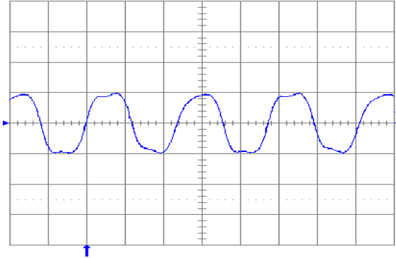
Fig. 5.0V.13: Output voltage ripple (20 mV/div.) at full rated load current into a resistive load with C_o = 10 \mu\text{F} tantalum + 1\mu\text{F} ceramic and V_{in} = 24 \text{ V} . Time scale: 1 \mu\text{s}/\text{div} .
