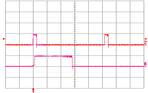
Fig. 2.0V.18: Load current (top trace, 20 A/div., 20 ms/div.) into a 10 mΩ short circuit during restart, at V_{in} = 24V . Bottom trace (20 A/div., 2 ms/div.) is an expansion of the on-time portion of the top trace.
