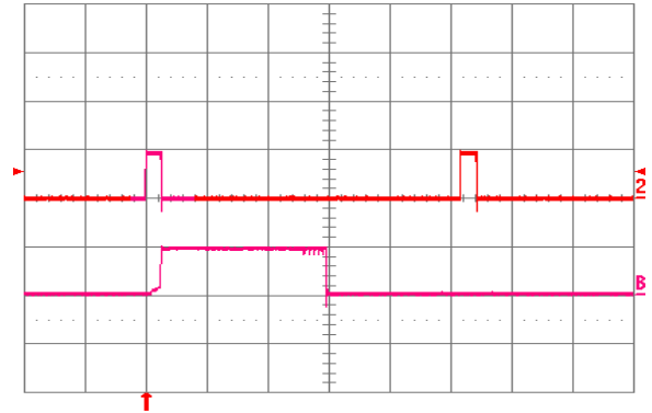
Fig. 1.2V.18: Load current (top trace, 20 A/div., 20 ms/div.) into a 10 mΩ short circuit during restart, at V_{in} = 24V . Bottom trace (20 A/div., 2 ms/div.) is an expansion of the on-time portion of the top trace.
