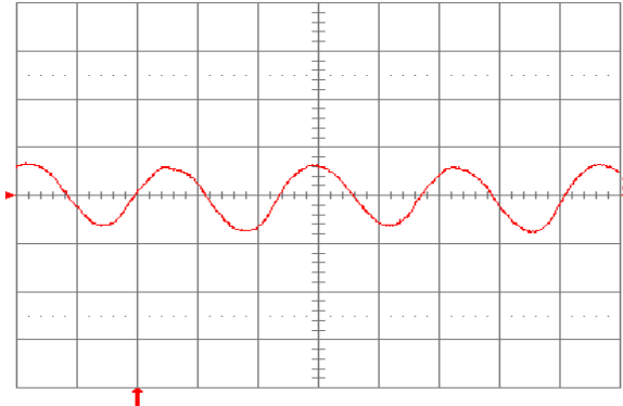
Fig. 5.0V.15: Input reflected ripple current, i_c (100 mA/div.), measured at input terminals at full rated load current and V_{in} = 24 \text{ V} . Refer to Fig. 5.0V.14 for test setup. Time scale: 1 \mu\text{s}/\text{div} .
