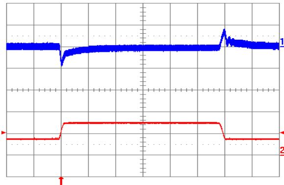
Fig. 1.8V.11: Output voltage response to load current step-change (3.75A – 7.5A – 3.75A) at V_{in} = 24V . Top trace: output voltage (100 mV/div.). Bottom trace: load current (5 A/div.). Current slew rate: 0.1 A/µs. C_o = 1 \mu F ceramic. Time scale: 0.2 ms/div.
