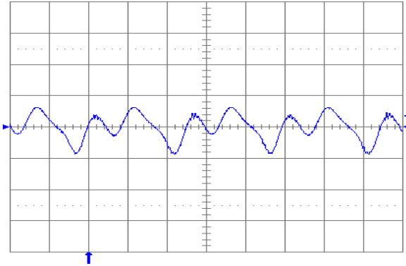
Fig. 1.2V.13: Output voltage ripple (20 mV/div.) at full rated load current into a resistive load with C_o = 10 \mu\text{F} tantalum + 1\mu\text{F} ceramic and V_{in} = 24 \text{ V} . Time scale: 1 \mu\text{s}/\text{div.}
