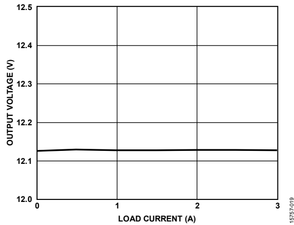
Figure 19. Load Regulation
