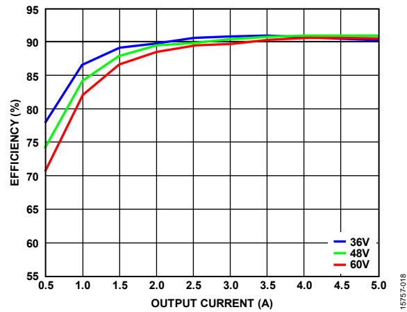
Figure 18. Efficiency Curves
