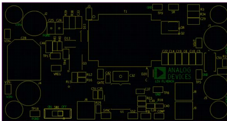
Figure 23. Silkscreen Top
