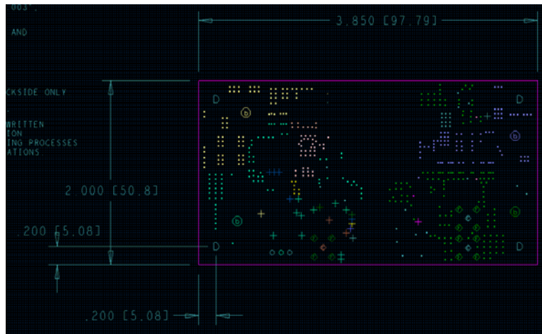
Figure 22. Board Outline
