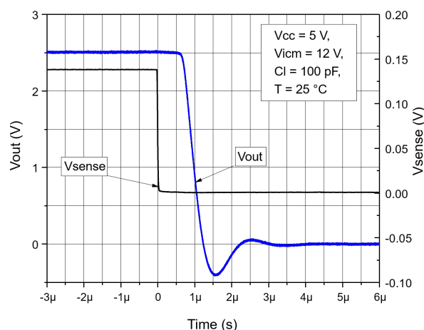
Figure 78. Positive overvoltage recovery V_{CC} = \pm 2.5\text{ V}
