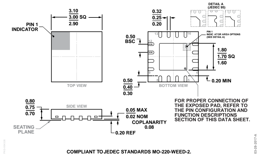
COMPLIANT TO JEDEC STANDARDS MO-220-WEED-2. Figure 18. 16-Lead Lead Frame Chip Scale Package [LFCSP] 3 mm × 3 mm Body and 0.75 mm Package Height (CP-16-35) Dimensions shown in millimeters
