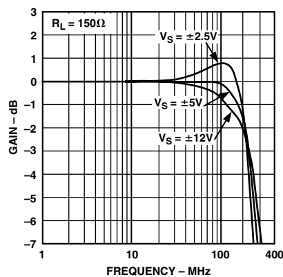
TPC 7. AD8130 Frequency Response vs. Supply, R_L = 150\text{ }\Omega
