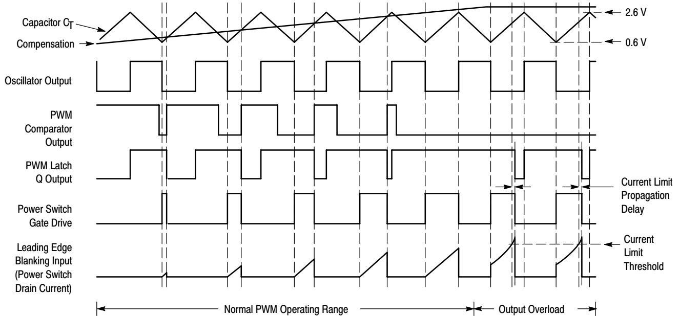
Figure 20. Timing Diagram
