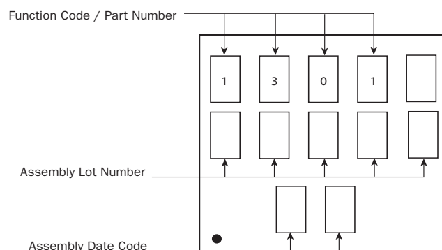
8 PIN MSOP PACKAGE
