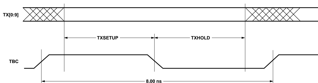
Figure 3b. Parallel transmitter section timing. TX_RATE = 0.
