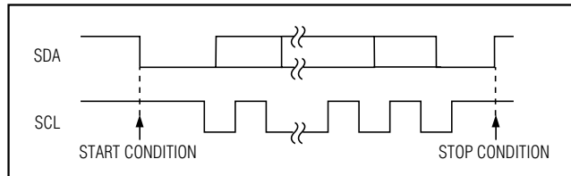
Figure 7. Start and Stop Conditions on a 2-Wire Interface
