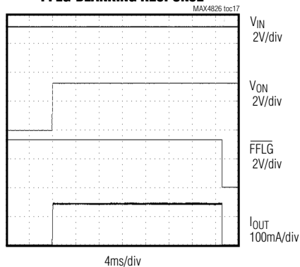
FFLG-BLANKING RESPONSE
