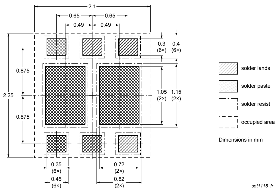
Fig. 19. Reflow soldering footprint for DFN2020-6 (SOT1118)
