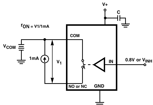
FIGURE 4. r_{ON} TEST CIRCUIT
