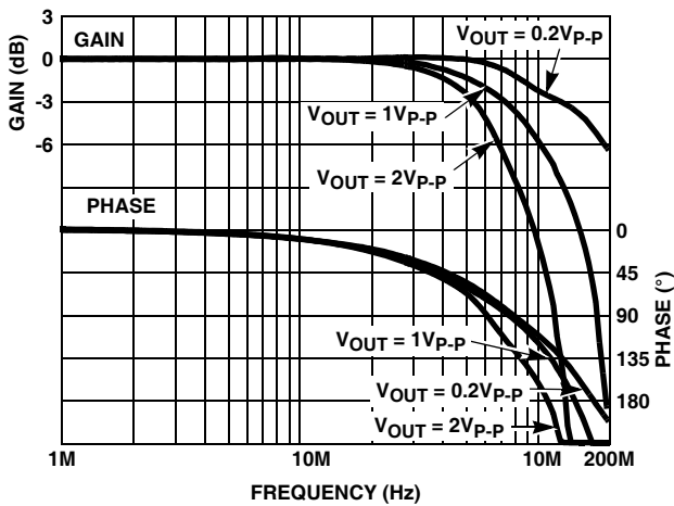
FIGURE 12. FREQUENCY RESPONSE
