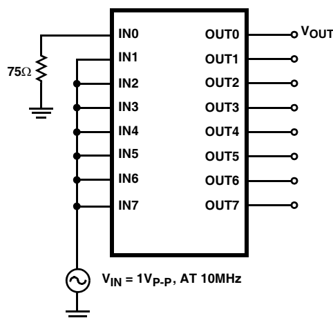
FIGURE 9. ALL HOSTILE CROSSTALK (NOTES 11, 16, 18 thru 20)
