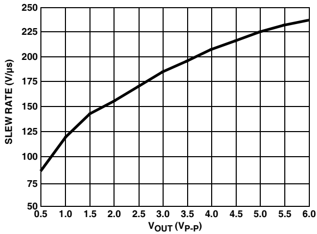
FIGURE 16. SLEW RATE vs V_{\text{OUT}}
