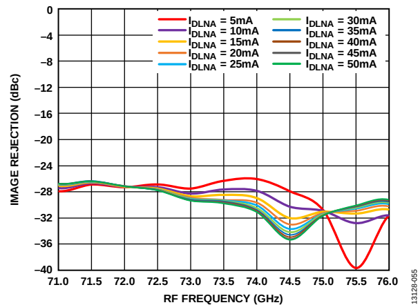
Figure 55. Image Rejection vs. RF Frequency at Various I_{DLNA} Values, RFIN = -20 dBm, LO = 2 dBm, IF = 500 MHz, V_{DLNA} = 3 V
