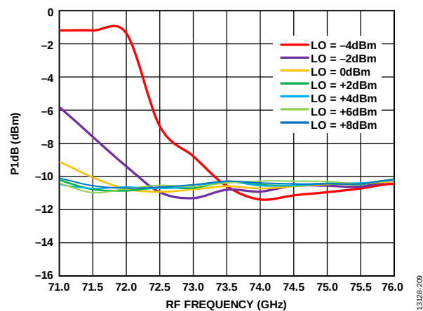
Figure 191. Input P1dB vs. RF Frequency at Various LO Powers, IF = 2000 MHz, V_{DLNA} = 4\text{ V}
