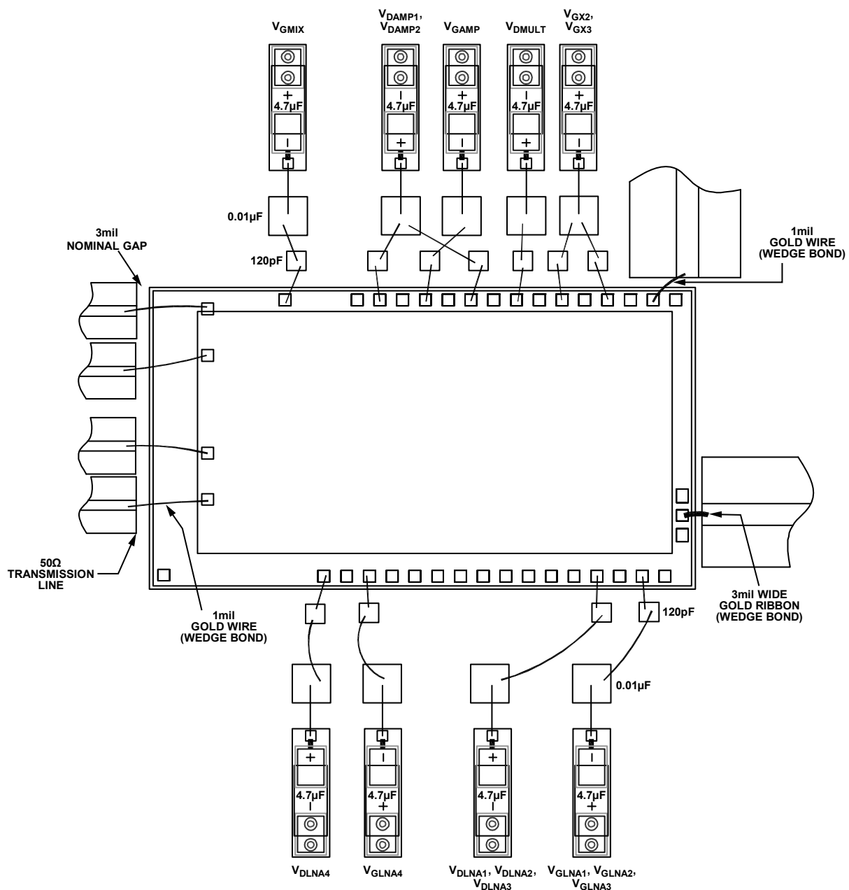
Figure 213. Assembly Diagram
