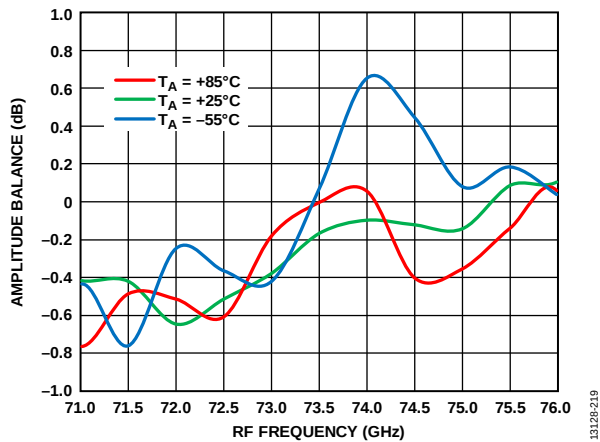
Figure 199. Amplitude Balance vs. RF Frequency at Various Temperatures, RFIN = -20 dBm, LO = 2 dBm, IF = 1000 MHz, V_{DLN} = 4 V
