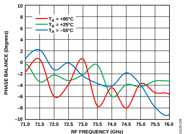
Figure 209. Phase Balance vs. RF Frequency at Various Temperatures, RFIN = -20 dBm, LO = 2 dBm, IF = 2000 MHz, V_{DLN} = 3 V
