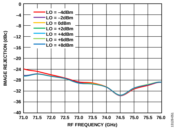
Figure 51. Image Rejection vs. RF Frequency at Various LO Powers, RFIN = -20 dBm, IF = 500 MHz, V_{DLNA} = 4 V
