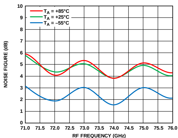
Figure 194. Noise Figure vs. RF Frequency at Various Temperatures, LO = 2 dBm, IF = 2000 MHz, V_{DLN} = 3 V
