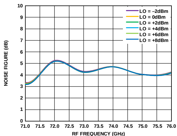
Figure 195. Noise Figure vs. RF Frequency at Various LO Powers, IF = 500 MHz, V_{DLN} = 3 V
