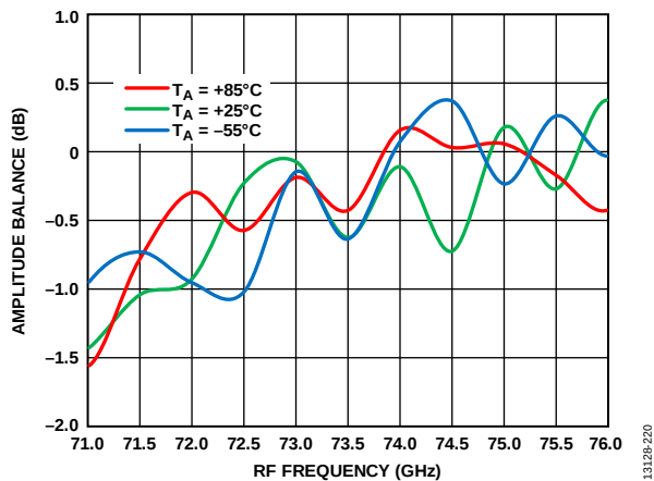
Figure 200. Amplitude Balance vs. RF Frequency at Various Temperatures, RFIN = -20 dBm, LO = 2 dBm, IF = 2000 MHz, V_{DLN} = 4 V
