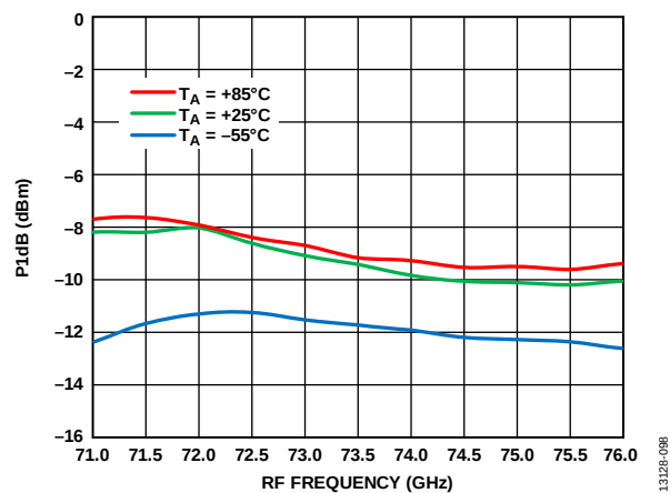
Figure 94. Input P1dB vs. RF Frequency at Various Temperatures, LO = 2\text{ dBm} , IF = 2000\text{ MHz} , V_{DLNA} = 4\text{ V}
