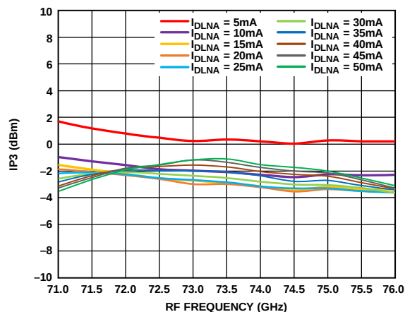
Figure 157. Input IP3 vs. RF Frequency at Various I_{DLNA} Values, R_{FIN} = -20 dBm, LO = 2 dBm, IF = 1000 MHz, V_{DLNA} = 3 V
