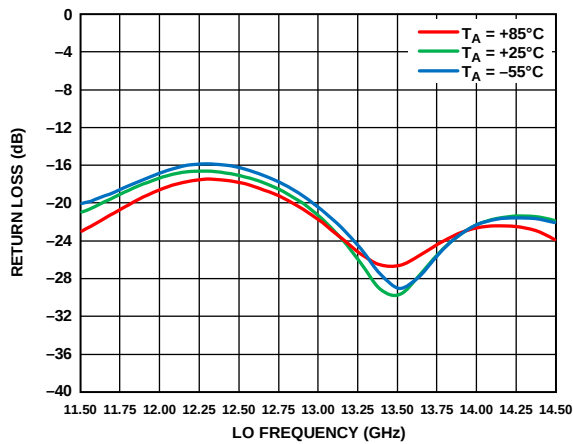
Figure 40. LO Return Loss vs. LO Frequency at Various Temperatures, LO = 2 dBm, V_{DLNA} = 4 V
