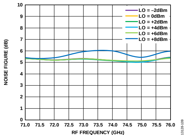
Figure 101. Noise Figure vs. RF Frequency at Various LO Powers, IF = 2000 MHz, V_{DLN} = 3 V
