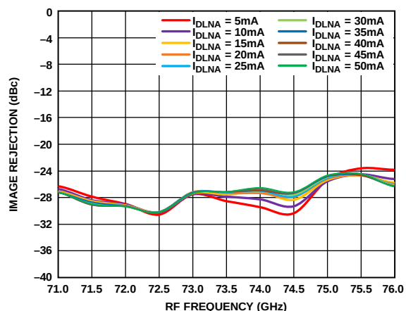
Figure 125. Image Rejection vs. RF Frequency at Various I_{DLNA} Values, RFIN = -20 dBm, LO = 2 dBm, IF = 500 MHz, V_{DLNA} = 3 V
