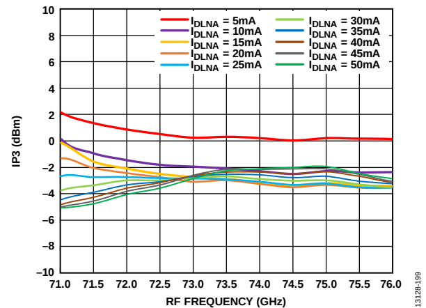
Figure 183. Input IP3 vs. RF Frequency at Various I_{DLNA} Values, RFIN = -20 dBm, LO = 2 dBm, IF = 2000 MHz, V DLNA = 3 V
