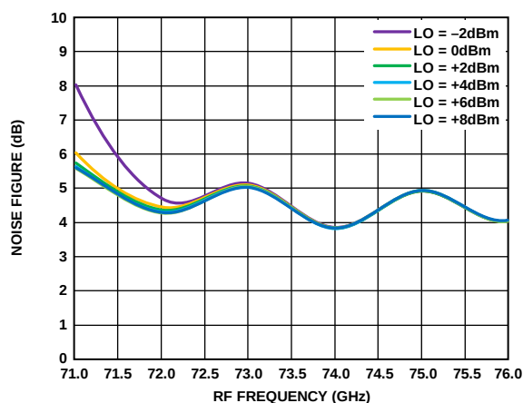
Figure 197. Noise Figure vs. RF Frequency at Various LO Powers, IF = 2000 MHz, V_{DLN} = 3 V
