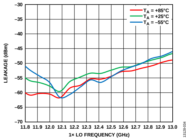
Figure 34. LO Leakage at IFOUT vs. 1 \times LO Frequency at Various Temperatures, LO = 2 dBm, V_{DLNA} = 3 V
