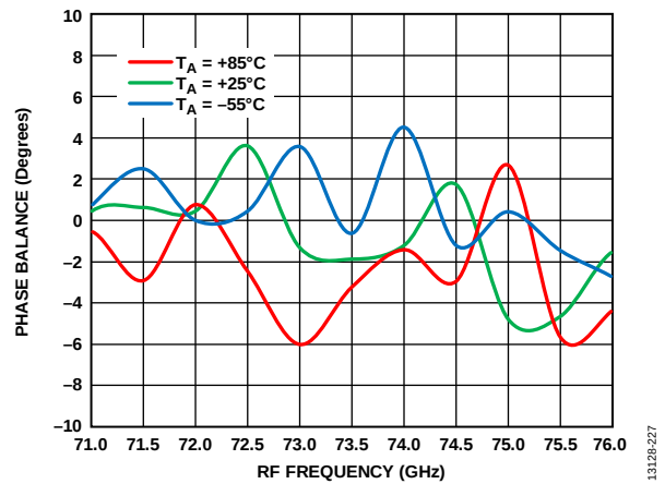
Figure 207. Phase Balance vs. RF Frequency at Various Temperatures, RFIN = -20 dBm, LO = 2 dBm, F = 500 MHz, V_{DLN} = 3 V
