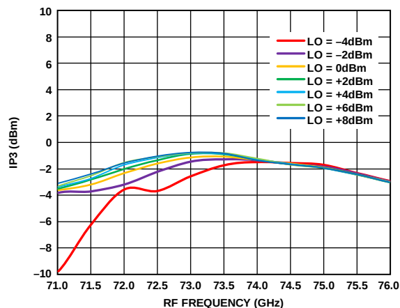
Figure 156. Input IP3 vs. RF Frequency at Various LO Powers, R_{FIN} = -20 dBm, IF = 1000 MHz, V_{DLNA} = 3 V
