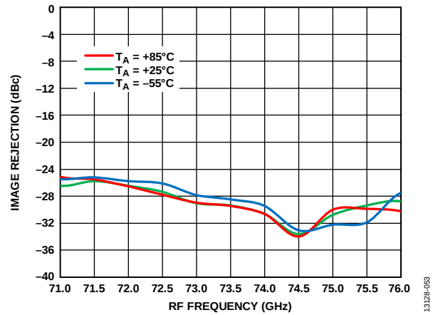
Figure 53. Image Rejection vs. RF Frequency at Various Temperatures, RFIN = -20 dBm, LO = 2 dBm, IF = 500 MHz, V_{DLNA} = 3 V
