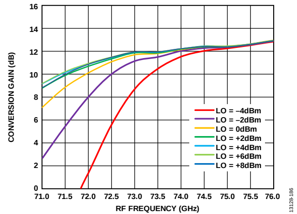
Figure 170. Conversion Gain vs. RF Frequency at Various LO Powers, R_{FIN} = -20 dBm, IF = 2000 MHz, V_{DLNA} = 3 V
