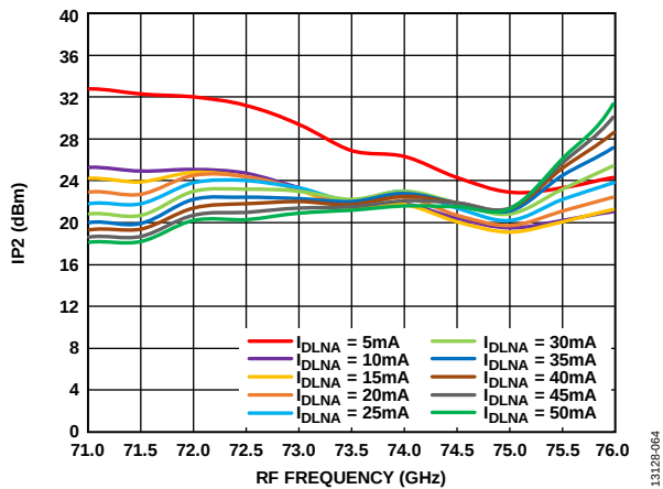
Figure 64. Input IP2 vs. RF Frequency at Various I_{DLNA} Values, RFIN = -20 dBm, LO = 2 dBm, IF = 500 MHz, V_{DLNA} = 4 V
