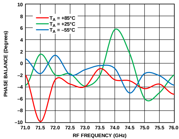
Figure 204. Phase Balance vs. RF Frequency at Various Temperatures, RFIN = -20 dBm, LO = 2 dBm, IF = 500 MHz, V_{DLN} = 4 V
