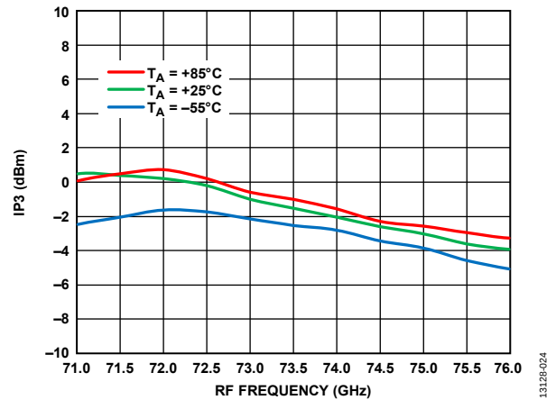
Figure 24. Input IP3 vs. RF Frequency at Various Temperatures, RFIN = -20 dBm, LO = 2 dBm, IF = 1000 MHz, V_{DLNA} = 3 V
