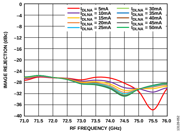
Figure 52. Image Rejection vs. RF Frequency at Various I_{DLNA} Values, RFIN = -20 dBm, LO = 2 dBm, IF = 500 MHz, V_{DLNA} = 4 V
