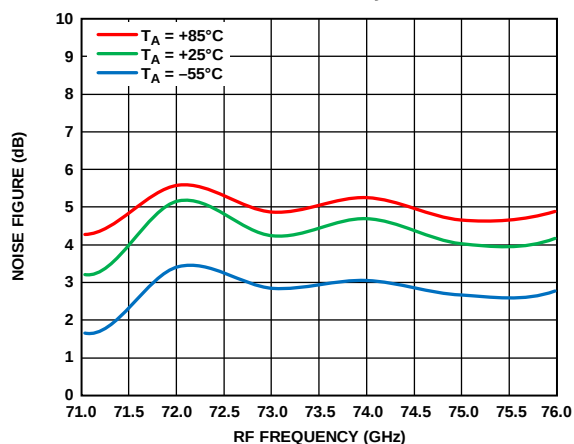
Figure 192. Noise Figure vs. RF Frequency at Various Temperatures, LO = 2 dBm, IF = 500 MHz, V_{DLN} = 3 V
