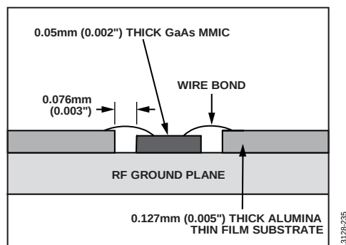
Figure 214. Routing RF Signals
