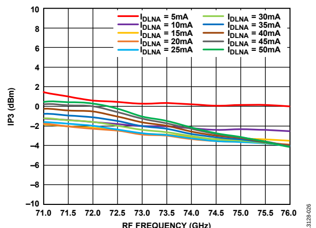
Figure 26. Input IP3 vs. RF Frequency at Various I_{DLNA} Values, RFIN = -20 dBm, LO = 2 dBm, IF = 1000 MHz, V_{DLNA} = 3 V
