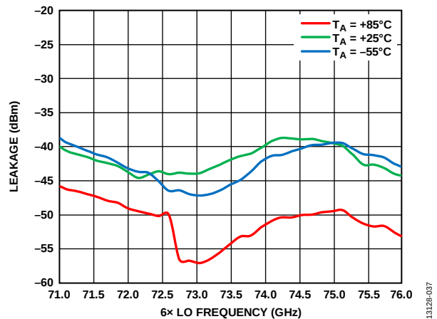
Figure 37. 6 \times LO Leakage at RFIN vs. 6 \times LO Frequency at Various Temperatures, LO = 2 dBm, V_{DLNA} = 3 V
