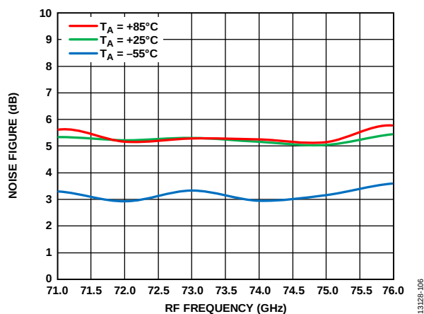
Figure 98. Noise Figure vs. RF Frequency at Various Temperatures, LO = 2 dBm, IF = 2000 MHz, V_{DLN} = 3 V
