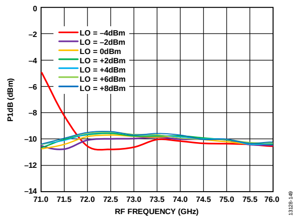
Figure 139. Input P1dB vs. RF Frequency at Various LO Powers, IF = 500 MHz, V_{DLNA} = 4\text{ V}
