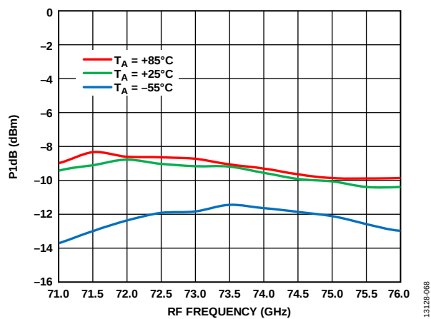
Figure 68. Input P1dB vs. RF Frequency at Various Temperatures, LO = 2 dBm, IF = 500 MHz, V_{DLNA} = 4\text{ V}
