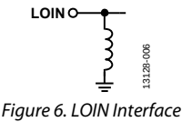
Figure 6. LOIN Interface
