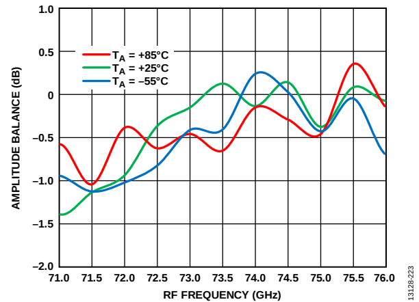
Figure 203. Amplitude Balance vs. RF Frequency at Various Temperatures, RFIN = -20 dBm, LO = 2 dBm, IF = 2000 MHz, V_{DLN} = 3 V
