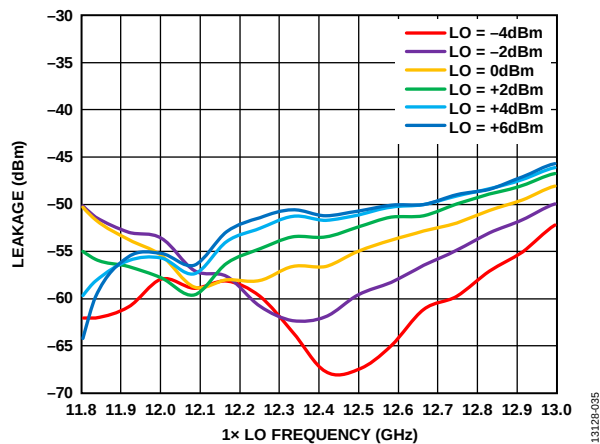
Figure 35. LO Leakage at IFOUT vs. 1 \times LO Frequency at Various LO Powers, V_{DLNA} = 3 V
