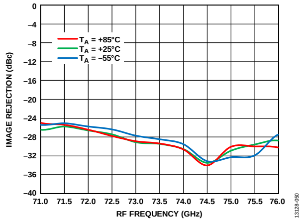
Figure 50. Image Rejection vs. RF Frequency at Various Temperatures, RFIN = -20 dBm, LO = 2 dBm, IF = 500 MHz, V_{DLNA} = 4 V
