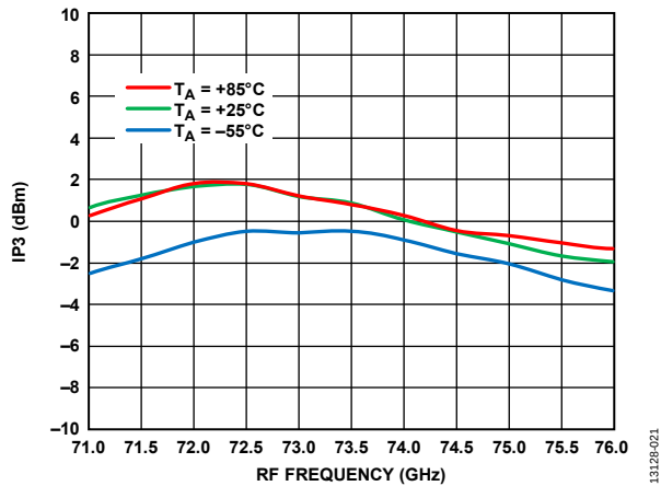
Figure 21. Input IP3 vs. RF Frequency at Various Temperatures, RFIN = -20 dBm, LO = 2 dBm, IF = 1000 MHz, V_{DLNA} = 4 V
