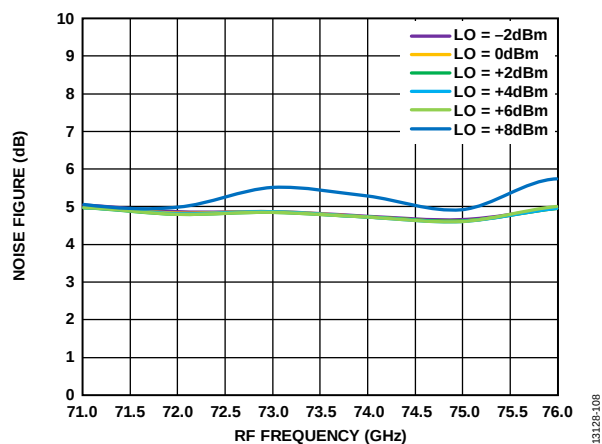
Figure 100. Noise Figure vs. RF Frequency at Various LO Powers, IF = 1000 MHz, V_{DLN} = 3 V
