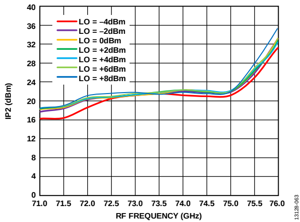
Figure 63. Input IP2 vs. RF Frequency at Various LO Powers, RFIN = -20 dBm, IF = 500 MHz, V_{DLNA} = 4 V
