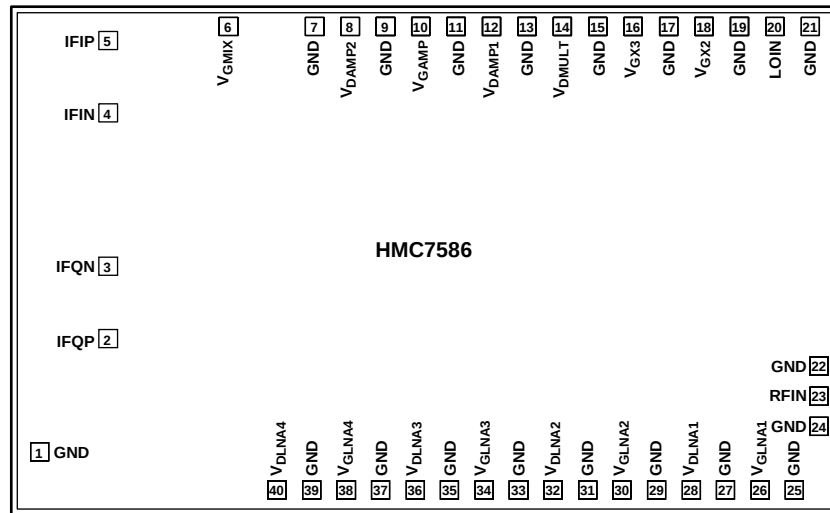
Figure 2. Pad Configuration
