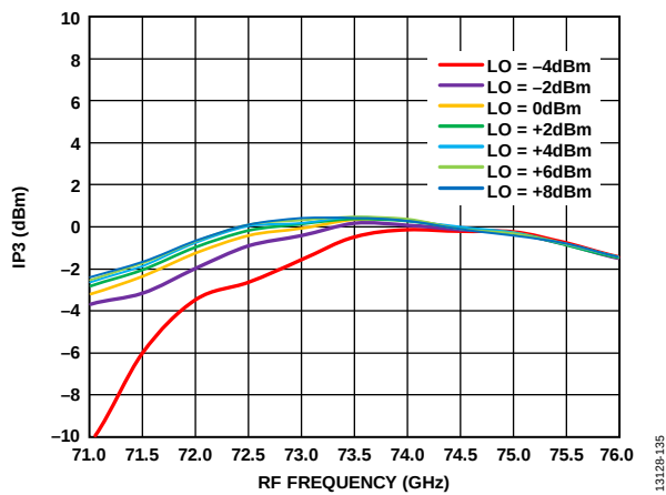
Figure 127. Input IP3 vs. RF Frequency at Various LO Powers, RFIN = -20 dBm, IF = 500 MHz, V_{DLNA} = 4 V
