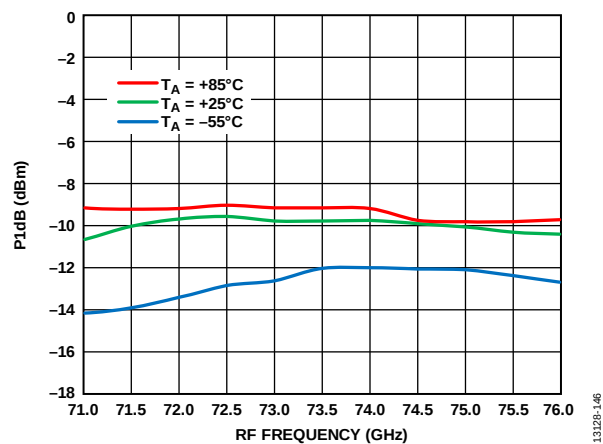
Figure 138. Input P1dB vs. RF Frequency at Various Temperatures, LO = 2 dBm, IF = 500 MHz, V_{DLNA} = 4\text{ V}
