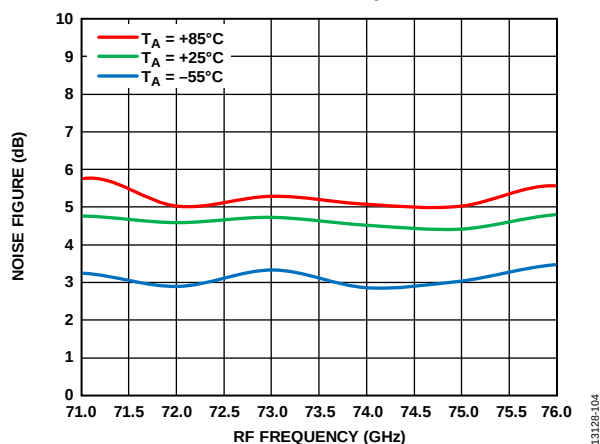
Figure 96. Noise Figure vs. RF Frequency at Various Temperatures, LO = 2 dBm, IF = 500 MHz, V_{DLN} = 3 V
