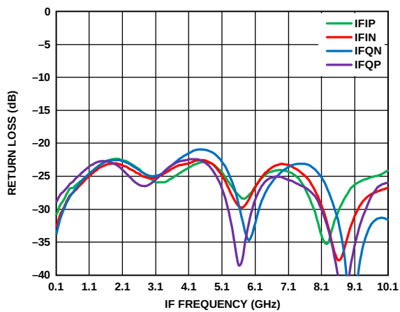
Figure 41. IF Return Loss vs. IF Frequency, LO = 2 dBm, LO = 12 GHz, V_{DLNA} = 4 V
