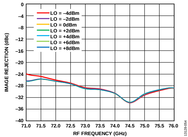
Figure 54. Image Rejection vs. RF Frequency at Various LO Powers, RFIN = -20 dBm, IF = 500 MHz, V_{DLNA} = 3 V
