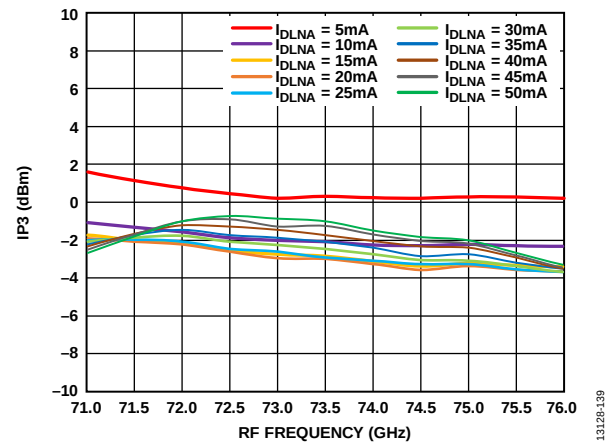
Figure 131. Input IP3 vs. RF Frequency at Various I_{DLNA} Values, RFIN = -20 dBm, LO = 2 dBm, IF = 500 MHz, V_{DLNA} = 3 V
