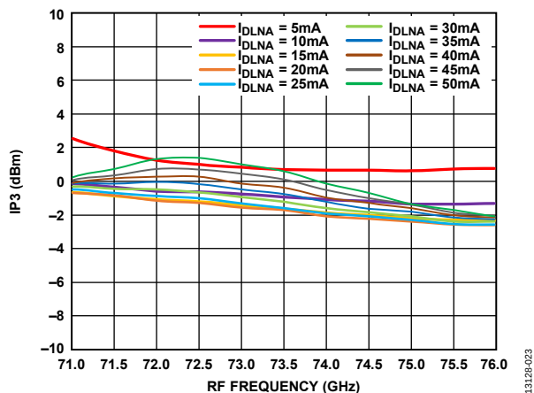
Figure 23. Input IP3 vs. RF Frequency at Various I_{DLNA} Values, RFIN = -20 dBm, LO = 2 dBm, IF = 1000 MHz, V_{DLNA} = 4 V
