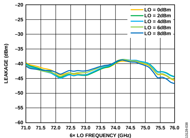
Figure 38. 6 \times LO Leakage at RFIN vs. 6 \times LO Frequency at Various LO Powers, V_{DLNA} = 3 V
