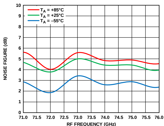
Figure 193. Noise Figure vs. RF Frequency at Various Temperatures, LO = 2 dBm, IF = 1000 MHz, V_{DLN} = 3 V
