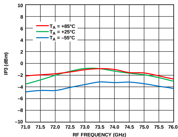
Figure 155. Input IP3 vs. RF Frequency at Various Temperatures, R_{FIN} = -20 dBm, LO = 2 dBm, IF = 1000 MHz, V_{DLNA} = 3 V
