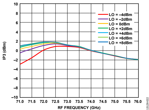
Figure 22. Input IP3 vs. RF Frequency at Various LO Powers, RFIN = -20 dBm, IF = 1000 MHz, V_{DLNA} = 4 V
