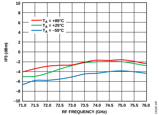
Figure 181. Input IP3 vs. RF Frequency at Various Temperatures, RFIN = -20 dBm, LO = 2 dBm, IF = 2000 MHz, V DLNA = 3 V
