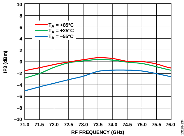
Figure 126. Input IP3 vs. RF Frequency at Various Temperatures, RFIN = -20 dBm, LO = 2 dBm, IF = 500 MHz, V_{DLNA} = 4 V
