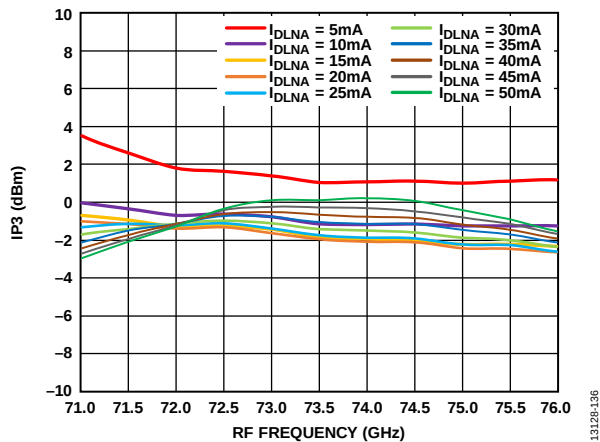
Figure 128. Input IP3 vs. RF Frequency at Various I_{DLNA} Values, RFIN = -20 dBm, LO = 2 dBm, IF = 500 MHz, V_{DLNA} = 4 V
