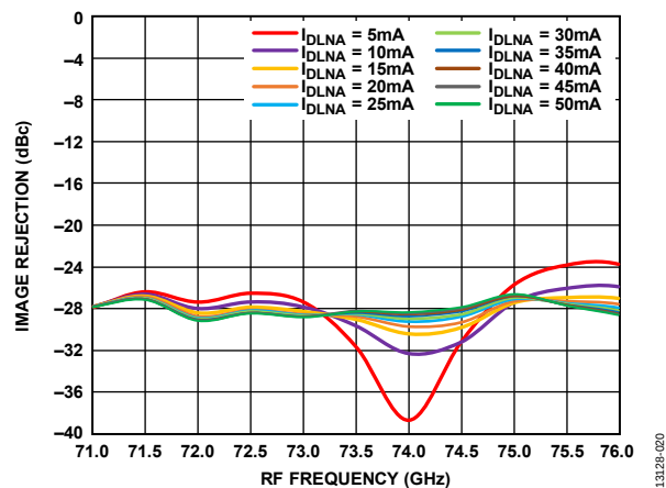
Figure 20. Image Rejection vs. RF Frequency at Various I_{DLNA} Values, R_{FIN} = -20 dBm, LO = 2 dBm, IF = 1000 MHz, V_{DLNA} = 3 V
