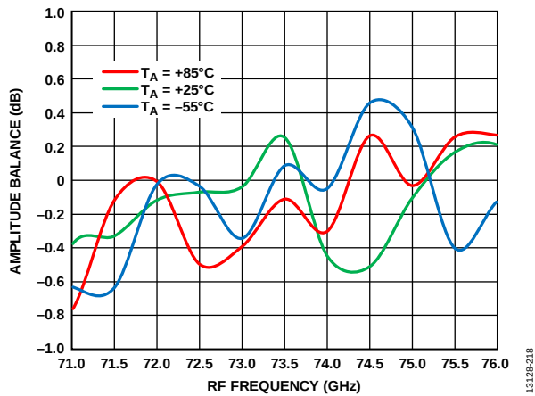
Figure 198. Amplitude Balance vs. RF Frequency at Various Temperatures, RFIN = -20 dBm, LO = 2 dBm, IF = 500 MHz, V_{DLN} = 4 V
