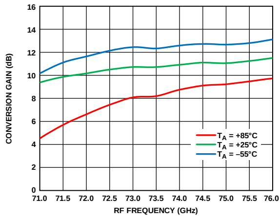
Figure 140. Conversion Gain vs. RF Frequency at Various Temperatures, R_{FIN} = -20 dBm, LO = 2 dBm, IF = 1000 MHz, V_{DLNA} = 4 V
