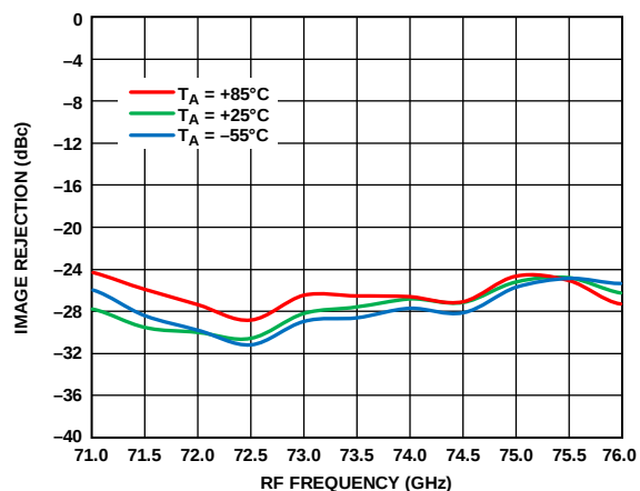
Figure 123. Image Rejection vs. RF Frequency at Various Temperatures, RFIN = -20 dBm, LO = 2 dBm, IF = 500 MHz, V_{DLNA} = 3 V
