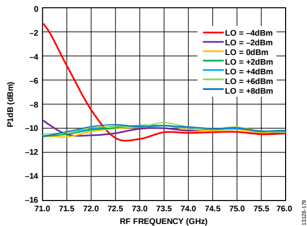
Figure 165. Input P1dB vs. RF Frequency at Various LO Powers, IF = 1000 MHz, V_{DLNA} = 4\text{ V}
