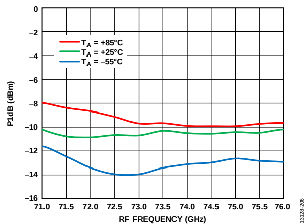
Figure 190. Input P1dB vs. RF Frequency at Various Temperatures, LO = 2 dBm, IF = 2000 MHz, V_{DLNA} = 4\text{ V}
