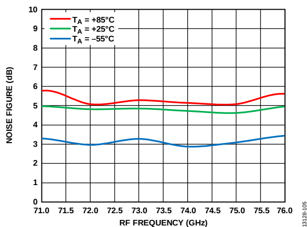
Figure 97. Noise Figure vs. RF Frequency at Various Temperatures, LO = 2 dBm, IF = 1000 MHz, V_{DLN} = 3 V
