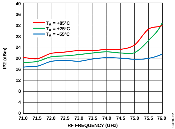
Figure 62. Input IP2 vs. RF Frequency at Various Temperatures, RFIN = -20 dBm, LO = 2 dBm, IF = 500 MHz, V_{DLNA} = 4 V
