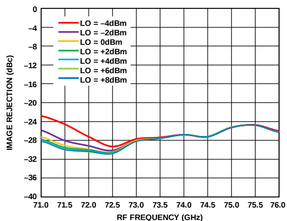
Figure 124. Image Rejection vs. RF Frequency at Various LO Powers, RFIN = -20 dBm, IF = 500 MHz, V_{DLNA} = 3 V
