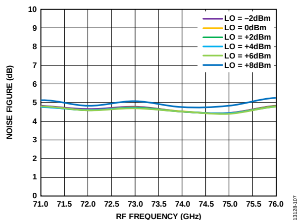
Figure 99. Noise Figure vs. RF Frequency at Various LO Powers, IF = 500 MHz, V_{DLN} = 3 V
