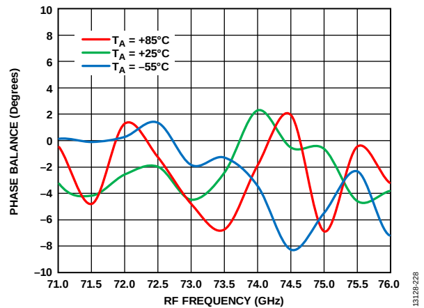
Figure 208. Phase Balance vs. RF Frequency at Various Temperatures, RFIN = -20 dBm, LO = 2 dBm, IF = 1000 MHz, V_{DLN} = 3 V
