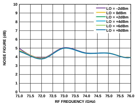
Figure 196. Noise Figure vs. RF Frequency at Various LO Powers, IF = 1000 MHz, V_{DLN} = 3 V
