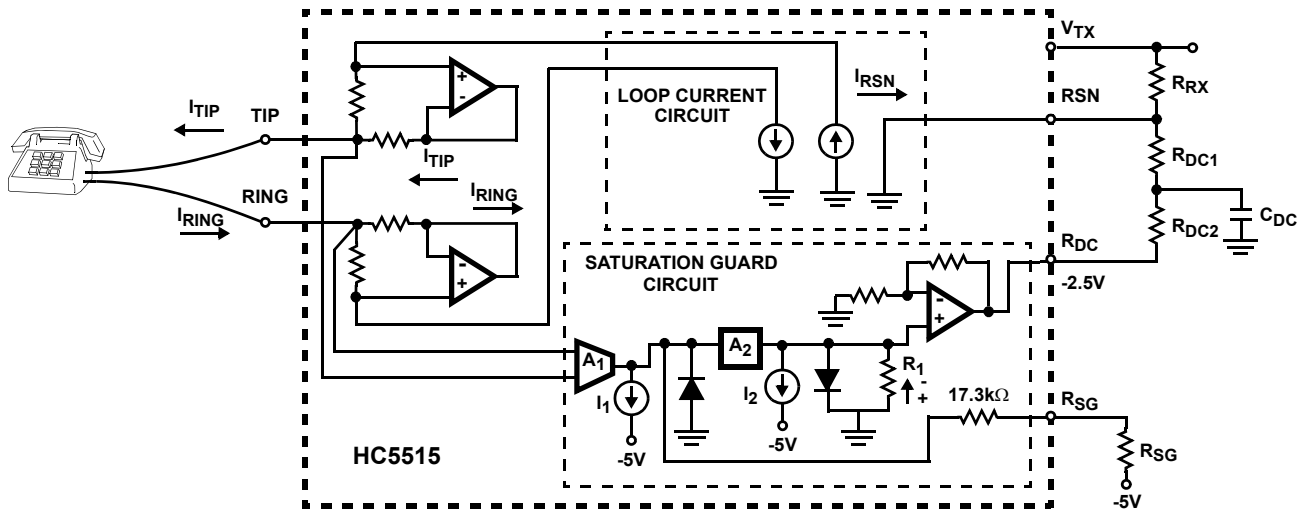
FIGURE 12. DC LOOP CURRENT
