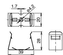
Mounting bracket LF9Z-1SB21
