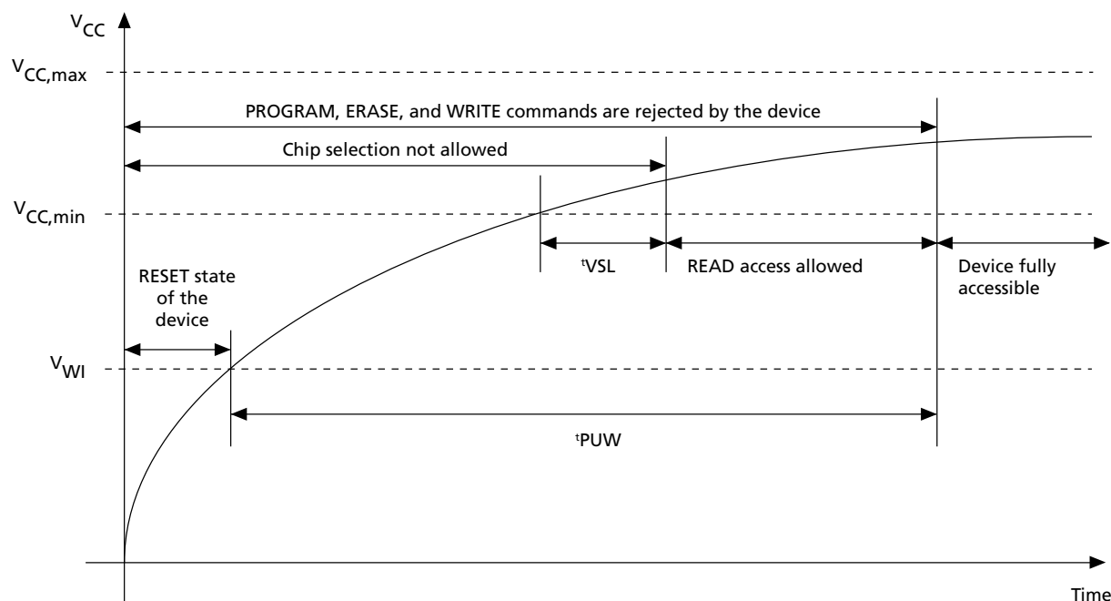
Figure 28: Power-Up Timing
