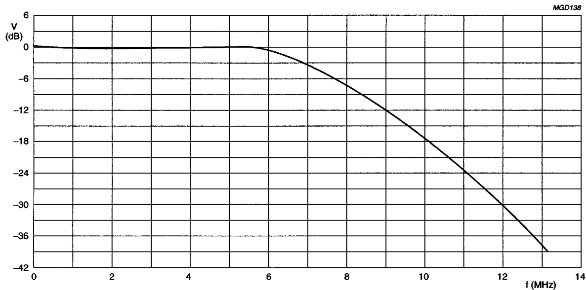
Fig.40 Anti-alias filter.
