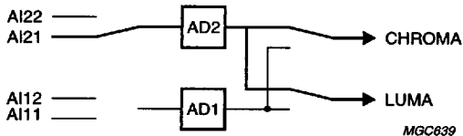
Fig.34 Mode 2; CVBS (automatic gain).
