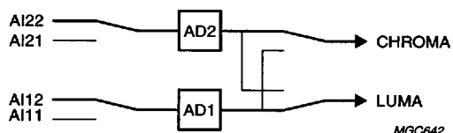
Fig.37 Mode 5 Y (automatic gain) + C (gain channel 2 fixed to GAI2 level).
