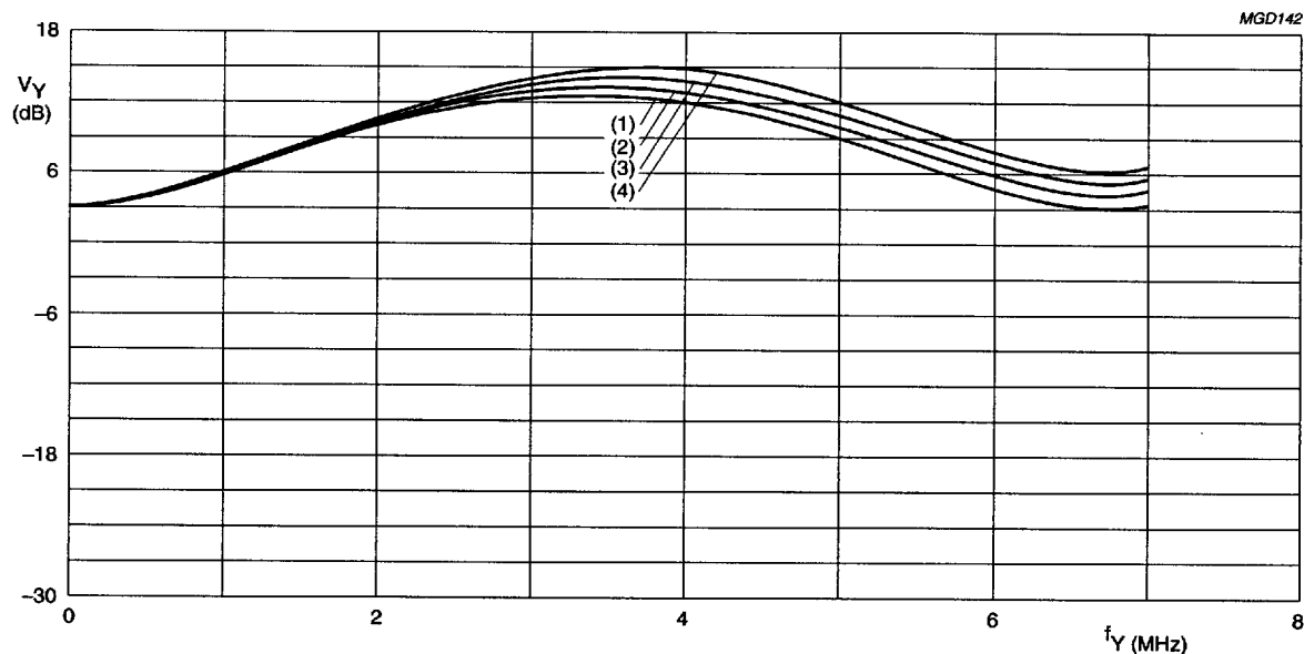
Fig. 45 Luminance control SA 09H, Y/C mode, prefilter on, different aperture factors.
