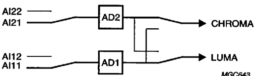
Fig.38 Mode 6 Y (automatic gain) + C (gain channel 2 adapted to Y gain).
