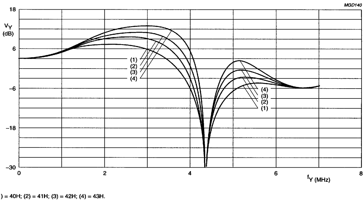
Fig.43 Luminance control SA 09H, 4.43 MHz Trap/CVBS mode, prefilter on, different aperture factors.
