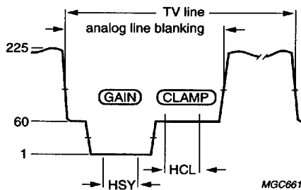
Fig.4 Analog line with clamp (HCL) and gain range (HSY).
