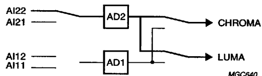
Fig.35 Mode 3; CVBS (automatic gain).
