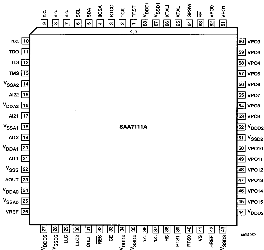
Fig.2 Pin configuration (PLCC68).
