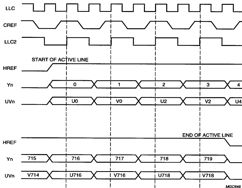
Fig.21 HREF timing diagram.
