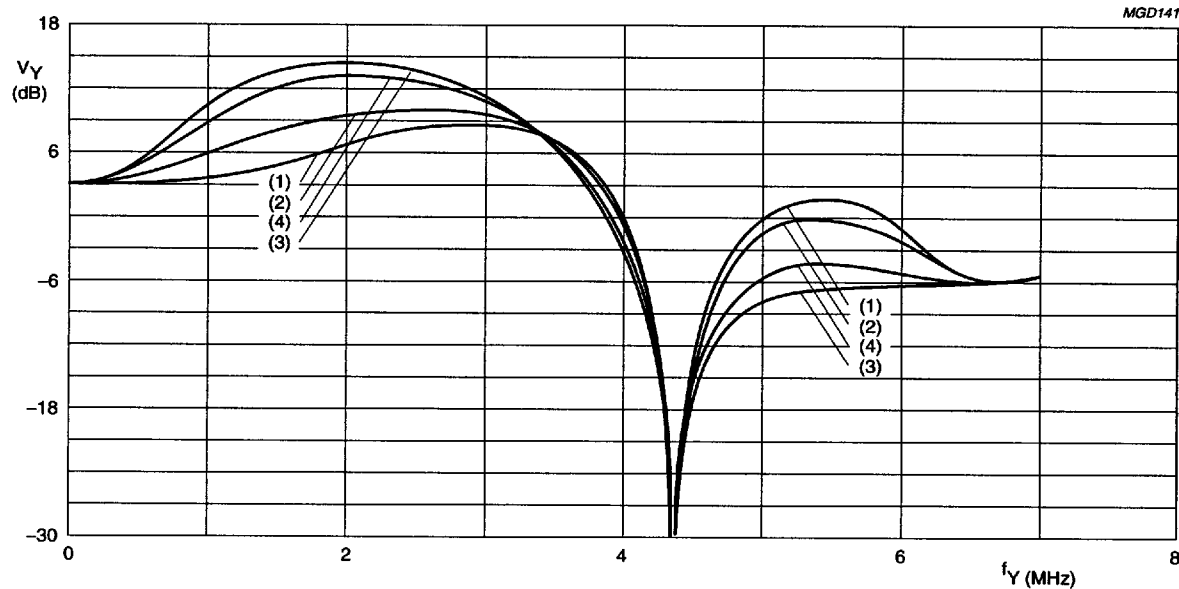
Fig. 44 Luminance control SA 09H, 4.43 MHz Trap/CVBS mode, prefilter off, different aperture band-pass centre frequencies.
