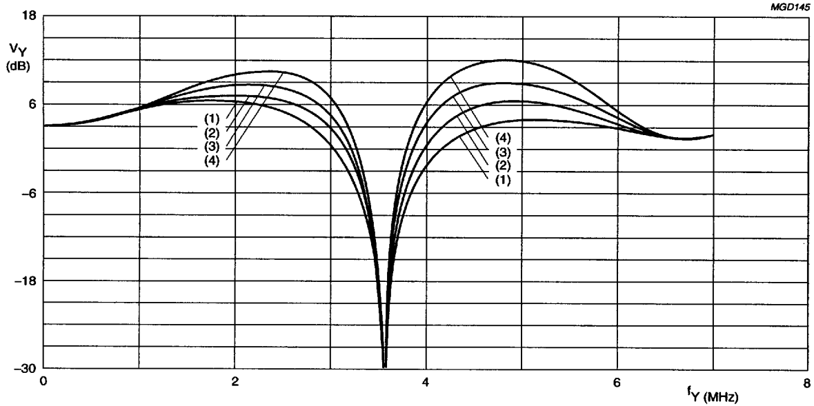
Fig.48 Luminance control SA 09H, 3.58 MHz Trap/CVBS mode, prefilter on, different aperture factors.
