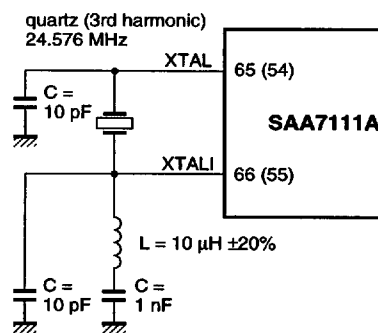
(a) With quartz crystal.
