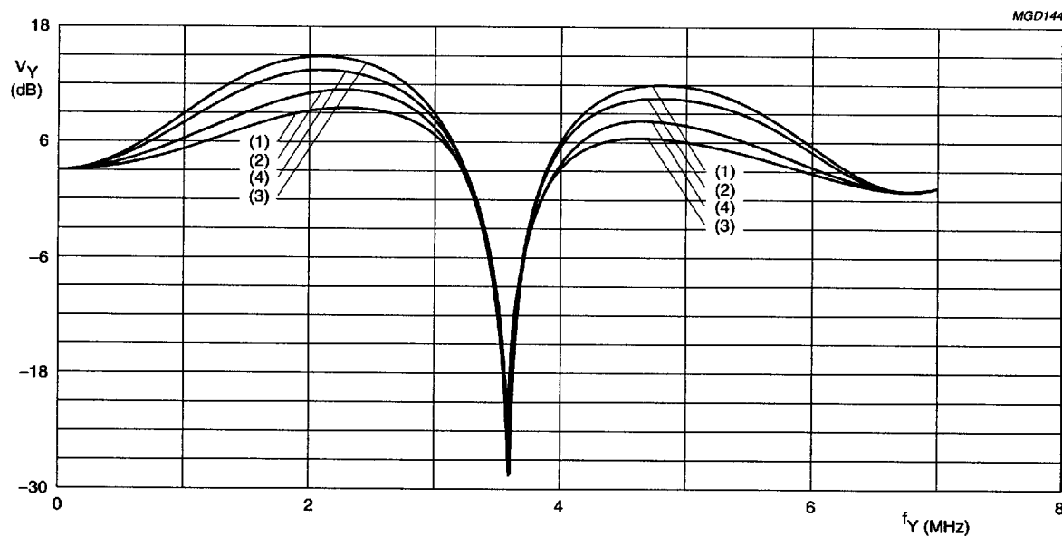
Fig.47 Luminance control SA 09H, 3.58 MHz Trap/CVBS mode, prefilter on, different aperture band-pass centre frequencies.
