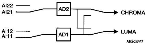
Fig.36 Mode 4 Y (automatic gain) + C (gain channel 2 fixed to GAI2 level).
