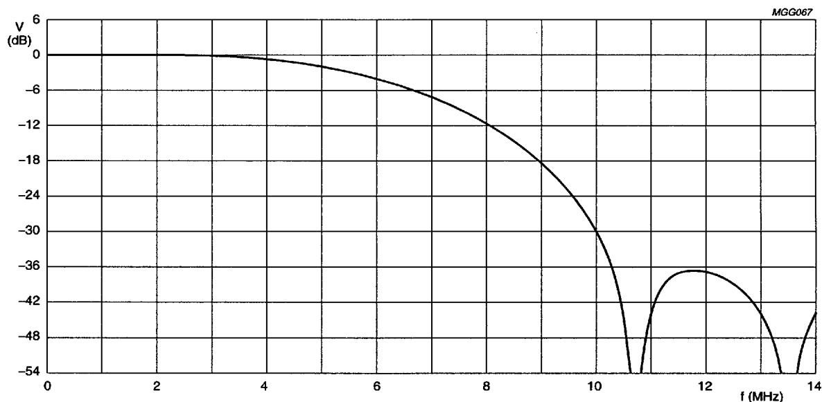
Fig.41 Interpolation filter for the upsampled CVBS-signal.
