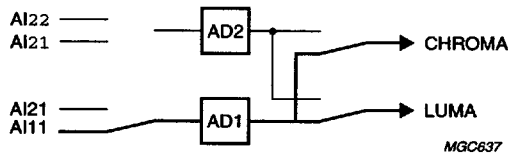
Fig.32 Mode 0; CVBS (automatic gain).
