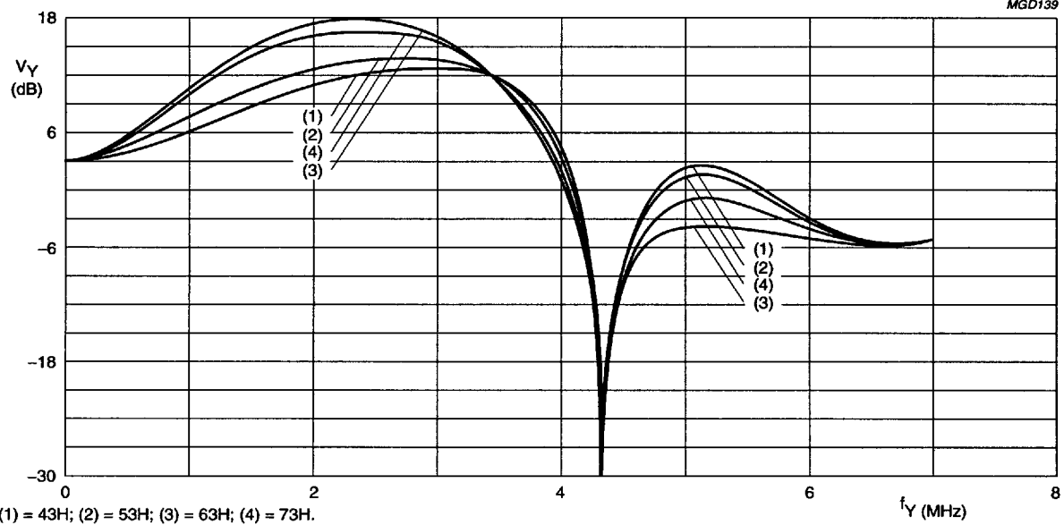
Fig.42 Luminance control SA 09H, 4.43 MHz Trap/CVBS mode, prefilter on, different aperture bandpass centre frequencies.
