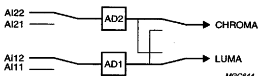
Fig.39 Mode 7 Y (automatic gain) + C (gain channel 2 adapted to Y gain).
