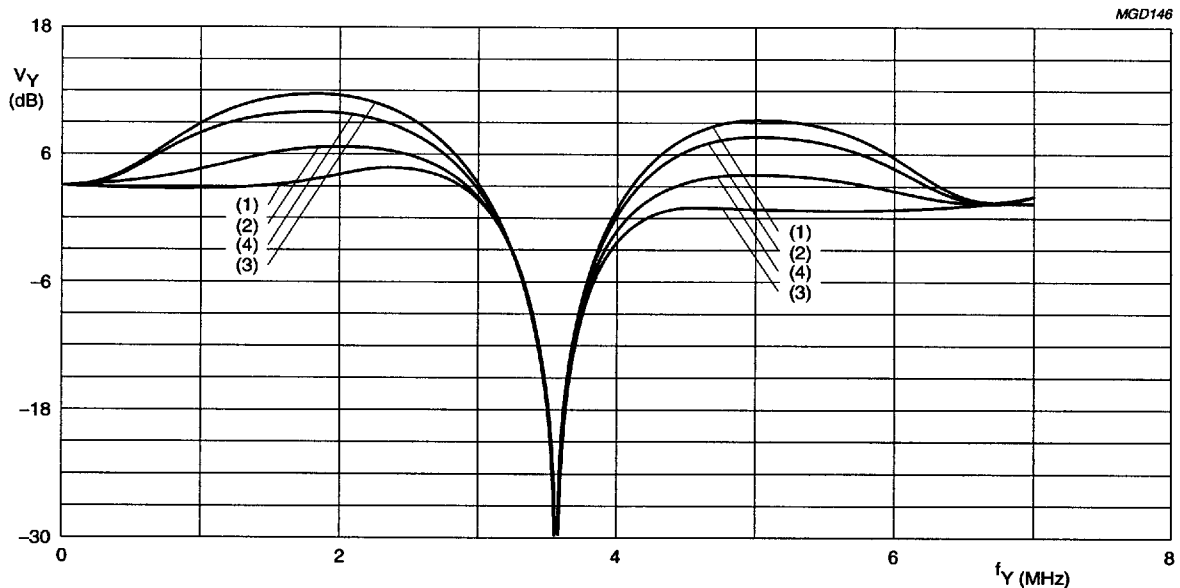
Fig.49 Luminance control SA 09H, 3.58 MHz Trap/CVBS mode, prefilter off, different aperture band-pass centre frequencies.
