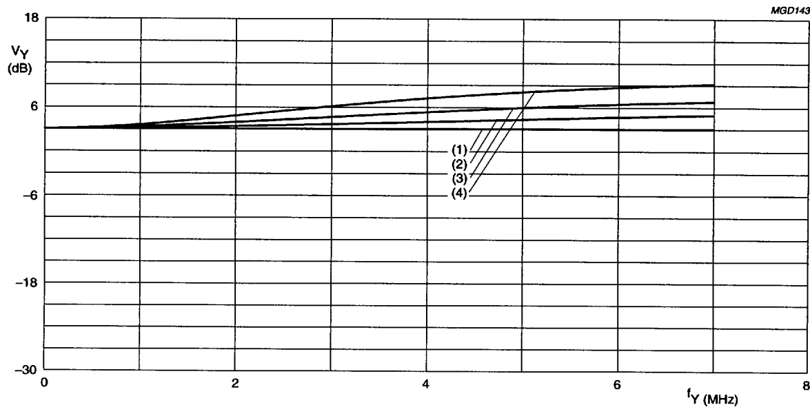
Fig.46 Luminance control SA 09H, Y/C mode, prefilter off, different aperture factors.
