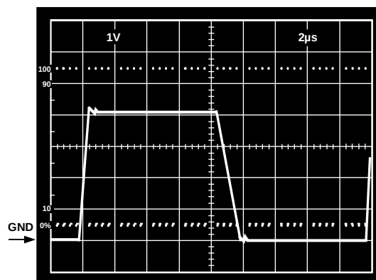
Figure 33. V_S = 5\text{ V} , 0\text{ V} ; Unity-Gain Follower Response to 0\text{ V} to 4\text{ V} Step
