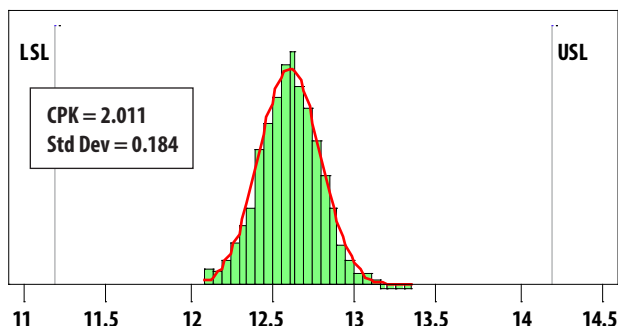
Figure 5. \text{Gain} ; LSL=11.2dB, Nominal = 12.6dB, USL=14.2dB
