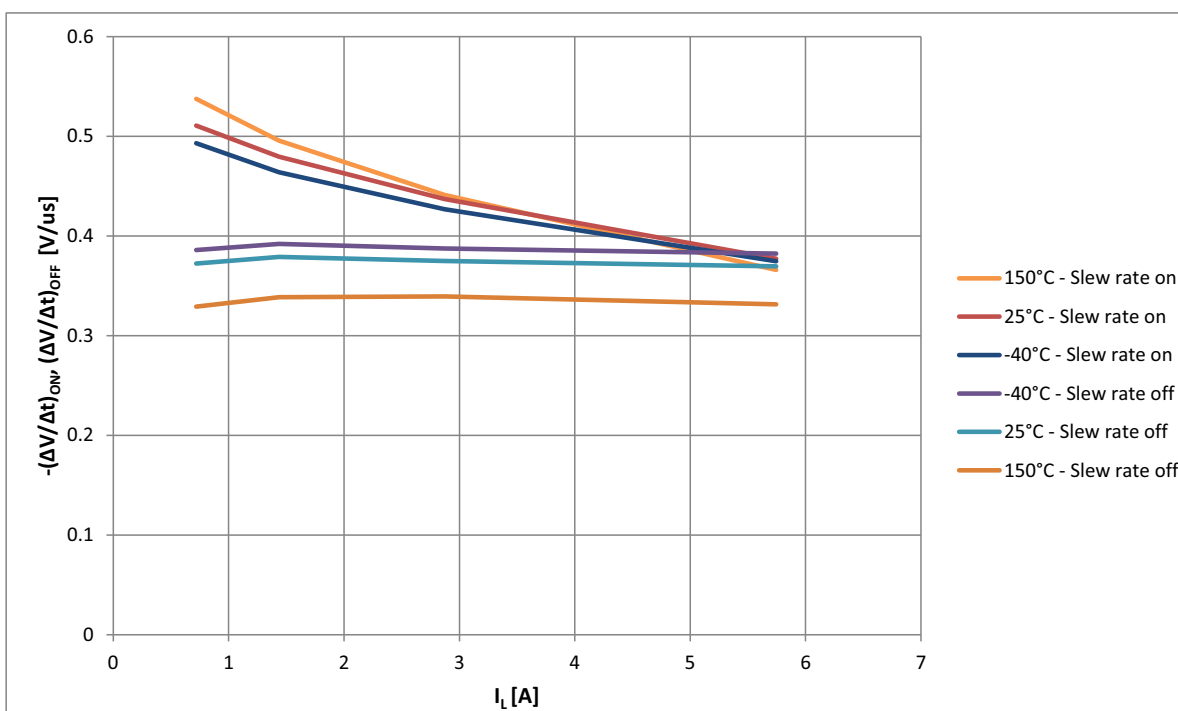
Figure 33 Typical -(\Delta V/\Delta t)_{ON} , (\Delta V/\Delta t)_{OFF} vs. I_L @ V_{IN} = 5V ; T_J = -40 \dots 150^\circ C
