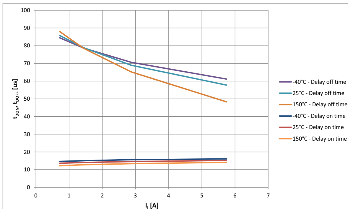
Figure 32 Typical t_{DON} , t_{DOFF} vs. I_L @ V_{IN} = 5V ; T_J = -40 \dots 150^\circ C
